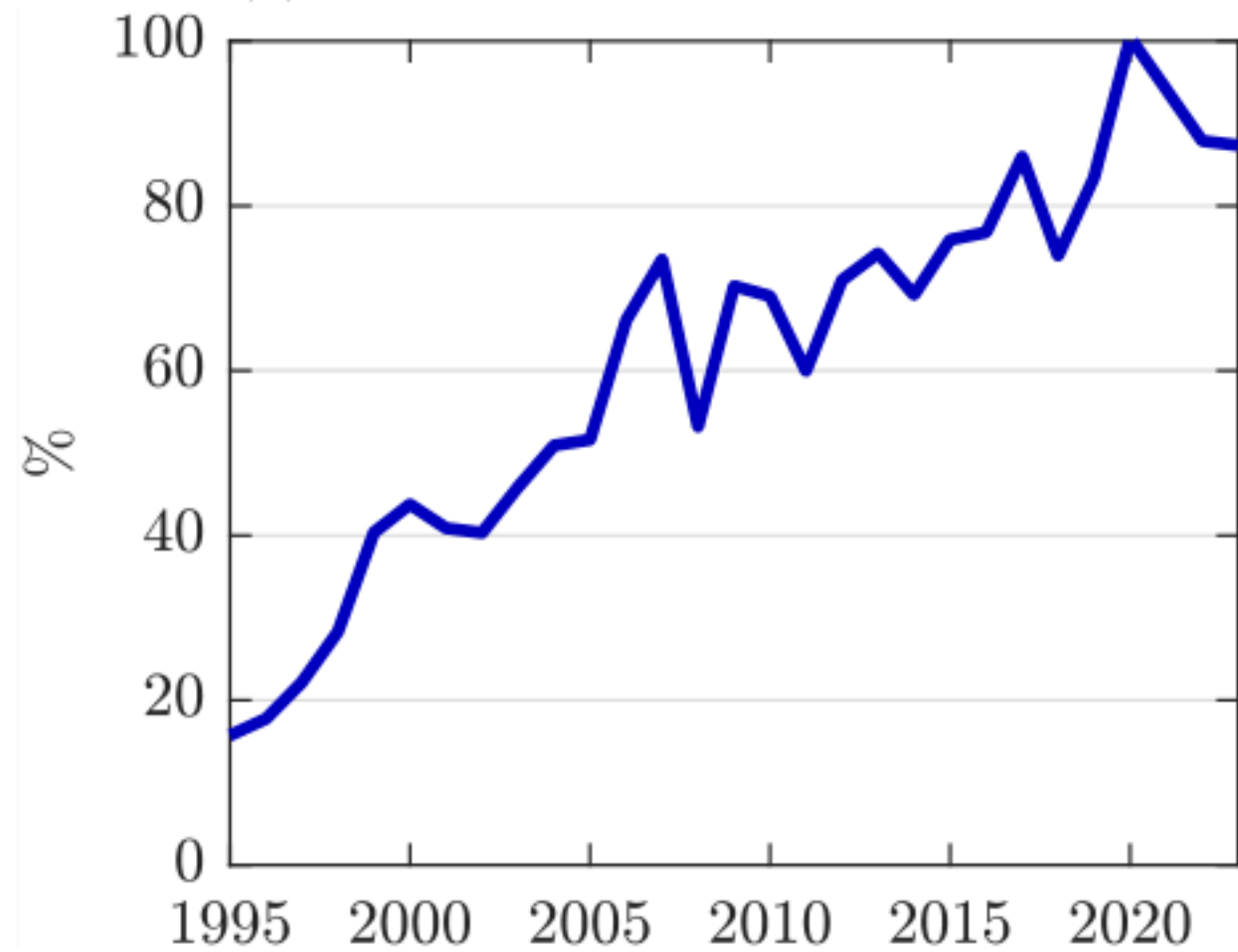
(a) Foreign holdings as % of GDP
