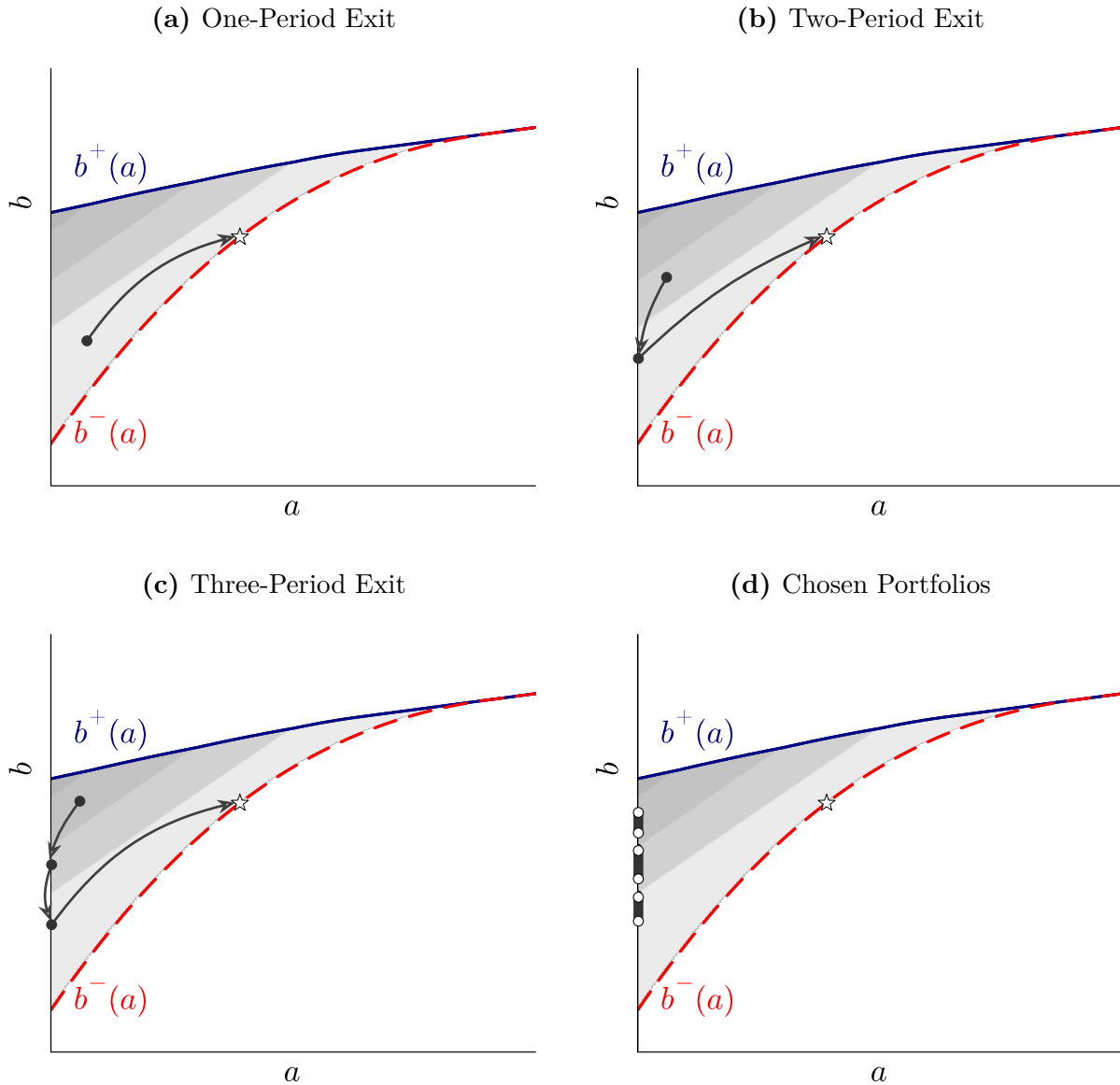
Figure 3: Periods to exit and portfolios. Panels (a)–(c) show cases where the government exits in one, two, and three periods, respectively. In panel (d), solid dots denote all portfolios chosen from initial positions in the crisis zone with a - b < a^* - b^* . The star marks (a^*, b^*) in all panels.
