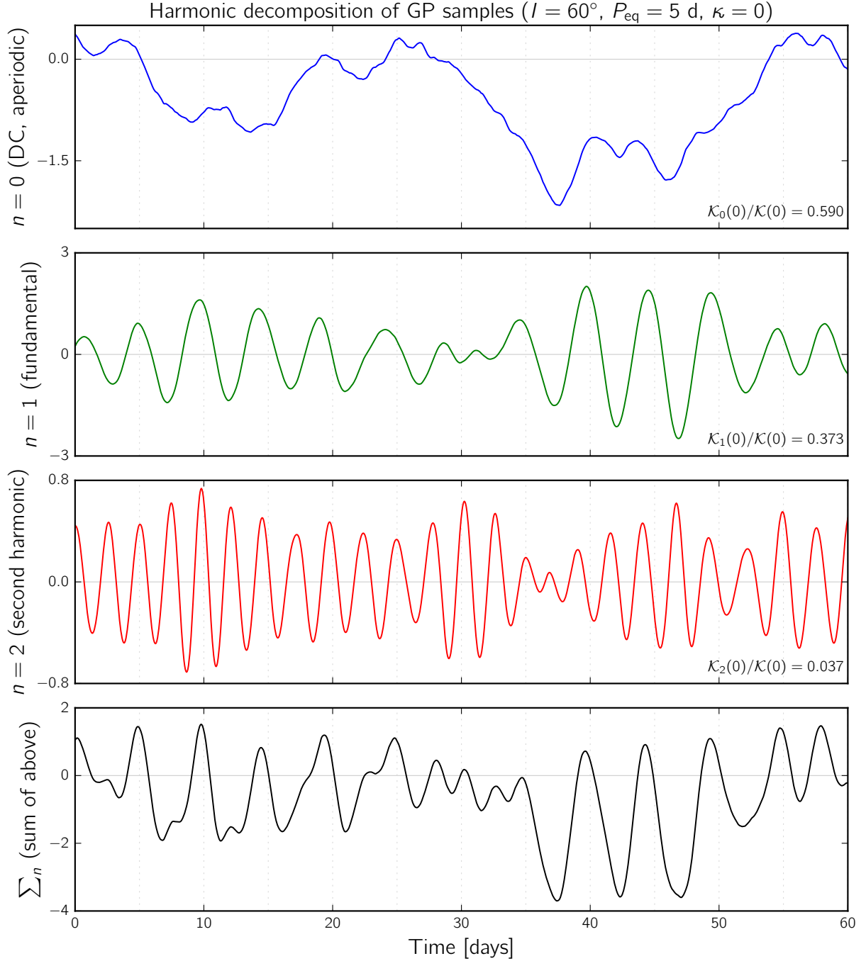
Figure 12. Harmonic decomposition of GP lightcurve samples ( I = 60^\circ , P_{\text{eq}} = 5 d, \kappa = 0 , \ell_{\text{spot}} = 15 d, \tau_{\text{spot}} = 3 d). Each of the top three panels is an independent draw from a single harmonic term \mathcal{K}_n of Eq. (70): the aperiodic n = 0 (spot emergence and decay), the fundamental n = 1 (rotational modulation at P_{\text{eq}} ), and the second harmonic n = 2 (at P_{\text{eq}}/2 ). Annotations give each order's share of the variance, \mathcal{K}_n(0)/\mathcal{K}(0) . Because the terms are independently samplable, their sum (fourth panel) is a draw from the full kernel.
