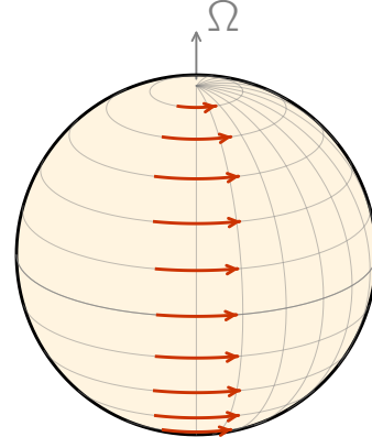
Anti-solar ( \kappa = -1.0 )
