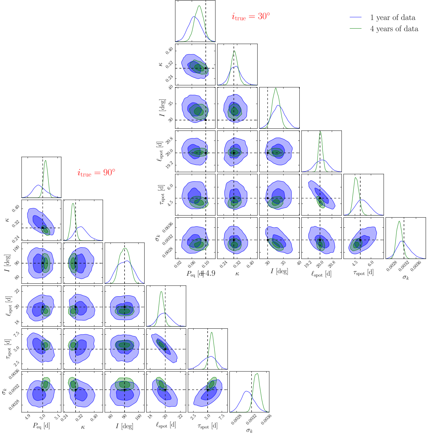
Figure 26. Posterior distributions for different inclinations: I = 90 (bottom left) and 30 (upper right) degrees based on nested sampling runs on synthetic lightcurves. The blue posterior outlines the constraints using 1 year of data, while the green posterior outlines the constraints using 4 years of data (comparable to the Kepler mission duration), and the true parameters are indicated by the dashed black lines. The posterior distributions show that the model can recover the true parameters with tight precision given a typical noise level of \sigma_n = 10^{-4} and a spot emergence rate of \dot{N}_{\text{spot}} = 0.25 \text{ d}^{-1} .
