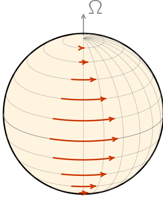
Solar-like ( \kappa = 1.0 )
