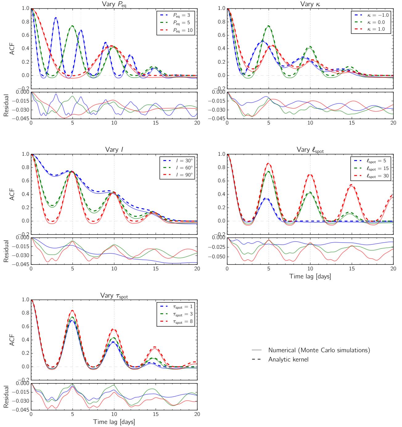
Figure 18. Analytic (dashed) vs. numerical Monte Carlo (solid) kernel comparison, parameter sweeps with varying P_{\text{eq}} (upper left), \kappa (upper right), inclination (middle left), \ell_{\text{spot}} (middle right), and \tau_{\text{spot}} (lower left). The numerical kernel is computed using N_{\text{sim}} = 500 lightcurve simulations with a baseline of 200d, and cadence of 0.05d. Vertical dotted lines mark the rotation frequency and its first harmonic.
