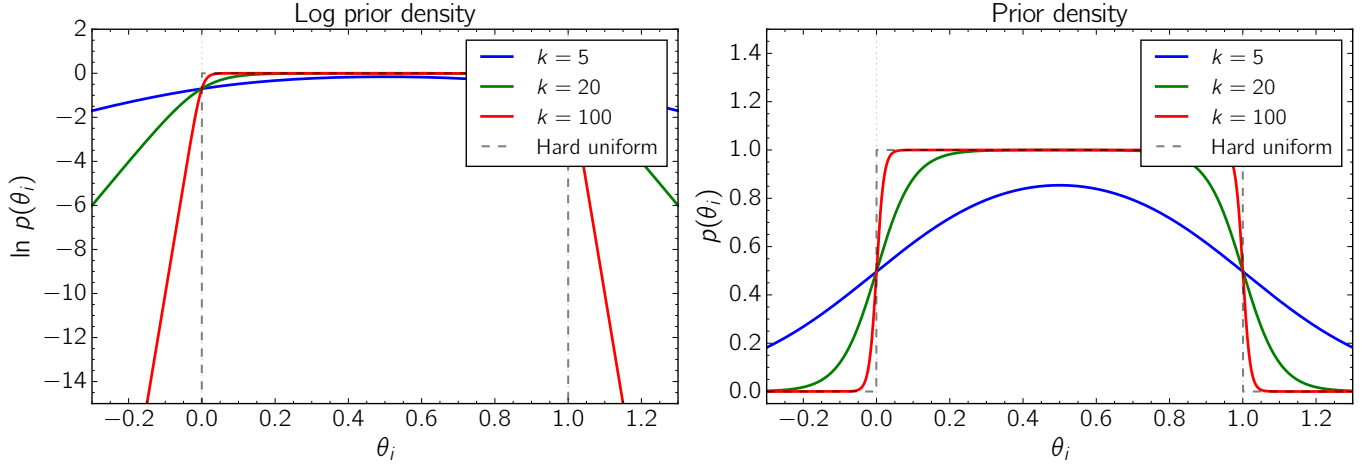
Figure 17. Soft uniform prior for a single parameter \theta with bounds [a, b] . The sigmoid-based formulation provides a smooth transition at the boundaries while maintaining an approximately uniform density within the bounds.
