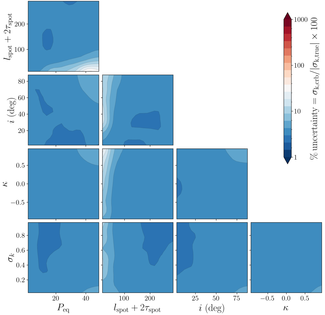
Figure 25. Same as Fig. 22, colored by \sigma_k .
