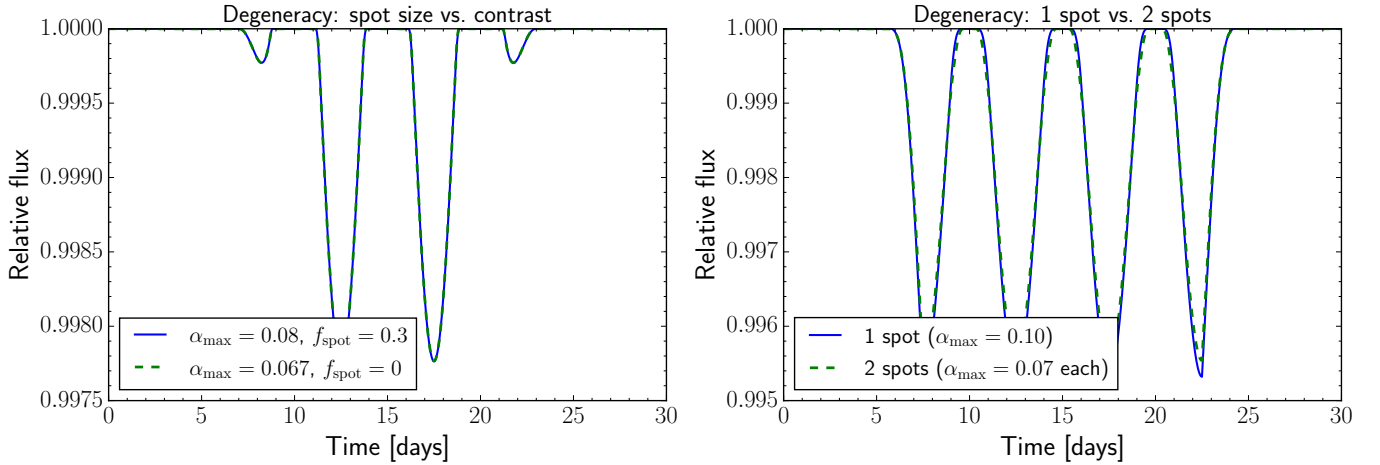
Figure 6. Illustration of degeneracies in starspot lightcurve modeling.
