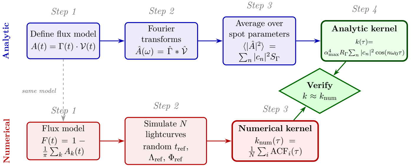
Figure 8. Overview of the kernel derivation strategy. Top row (blue): The analytic path derives k(\tau) from the single-spot flux model A(t) = \Gamma(t) \cdot \mathcal{V}(t) by (1) computing Fourier transforms of the envelope and visibility terms, (2) averaging the energy spectral density over random spot parameters ( t_{\text{ref}}, \Lambda_{\text{ref}}, \Phi_{\text{ref}} ), and (3) applying the Wiener–Khinchin theorem. Bottom row (red): The numerical path simulates N lightcurves from the same flux model with randomly drawn spot parameters and estimates the kernel as the sample-averaged autocorrelation. Center (green): The two paths converge, verifying the analytic kernel against the numerical estimate.
