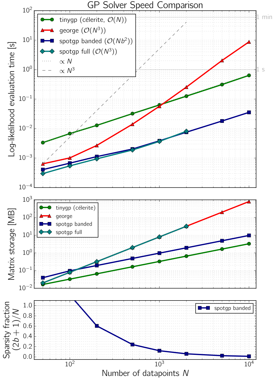
Figure 20. Benchmark of GP solver performance as a function of the number of datapoints N , using a one-sided exponential envelope with N_{\text{harm}} = 2 harmonics and cadence \Delta t = 1 d. Top: Wall-clock time for a single log-likelihood evaluation. tinygp (celerate, green) scales as \mathcal{O}(N) ; george (red) and spotgp full Cholesky (teal) scale as \mathcal{O}(N^3) ; spotgp banded (dark blue) scales as \mathcal{O}(Nb^2) . Horizontal gray lines mark 1 s and 1 min. Middle: Matrix storage in MB. The celerate and banded solvers scale linearly with N , while the dense solvers scale as N^2 . Bottom: Sparsity fraction (2b+1)/N of the banded covariance matrix, showing that the bandwidth b remains fixed as N grows. All JAX solvers are JIT-compiled and warmed up before timing.
