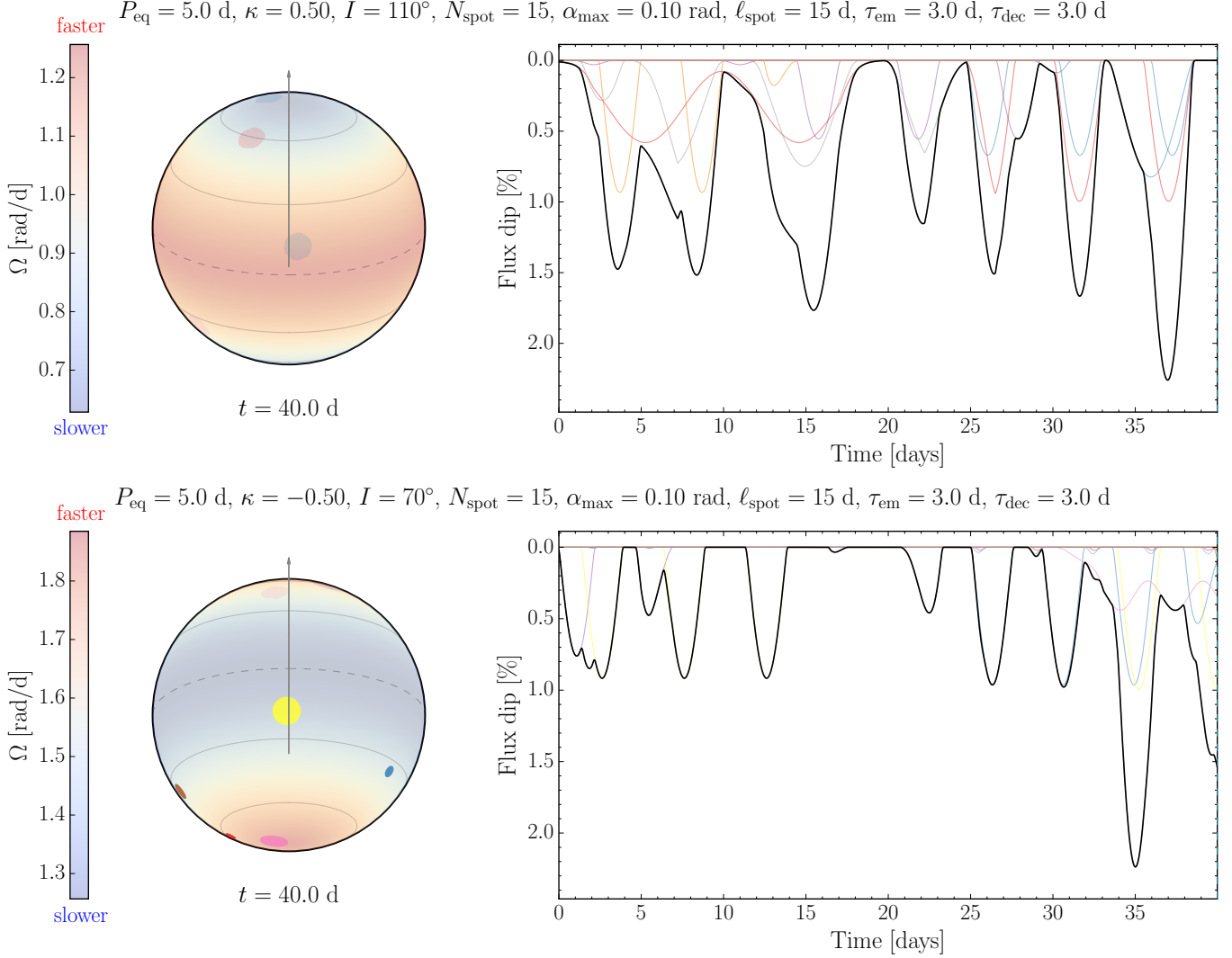
Figure 5. Examples of simulated lightcurves generated from the starspot model from the Kipping (2012) model. The top panel shows the case with solar-like differential rotation ( \kappa = 0.5 ), while the bottom panel shows the case with anti-solar differential rotation ( \kappa = -0.5 ). The contributions from each individual spot are shown in color, while the cumulative flux deficit is shown in black. The lightcurve exhibits quasi-periodic variability due to the rotation of the star and the emergence and decay of spots.
