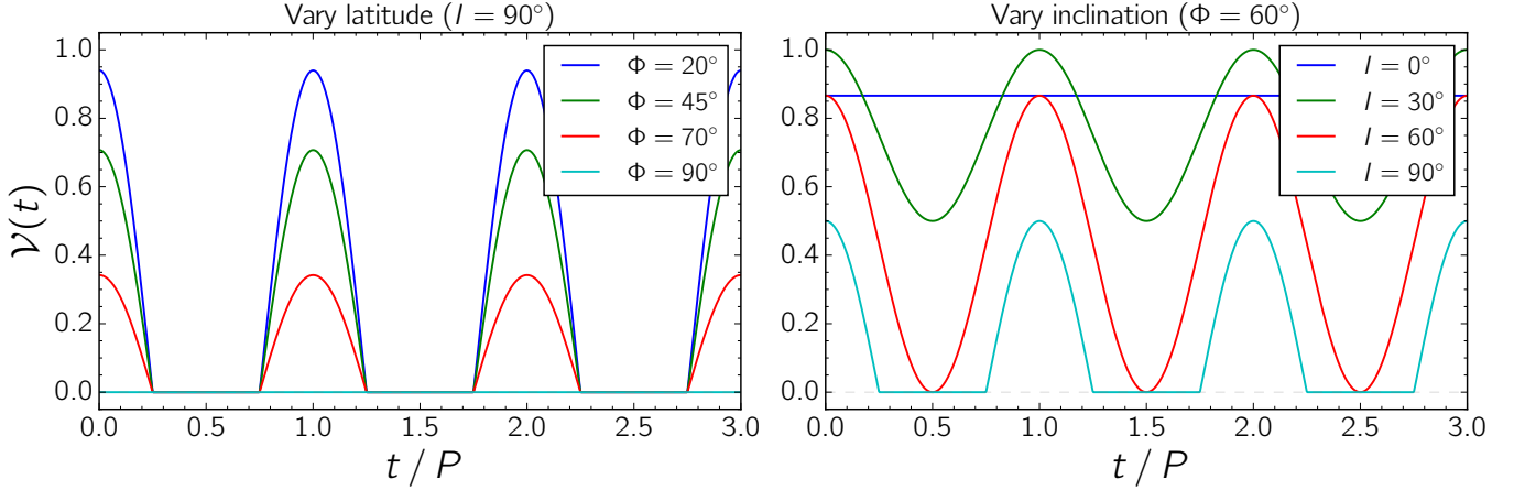
Figure 9. Visibility function \mathcal{V}(t) = \max\{\cos \beta(t), 0\} over three rotation periods. Left: varying spot latitude \Phi at fixed edge-on inclination I = 90^\circ . Right: varying stellar inclination I at fixed latitude \Phi = 60^\circ . The amplitude and duty cycle of \mathcal{V}(t) set the Fourier coefficients |c_n|^2 that enter the kernel.
