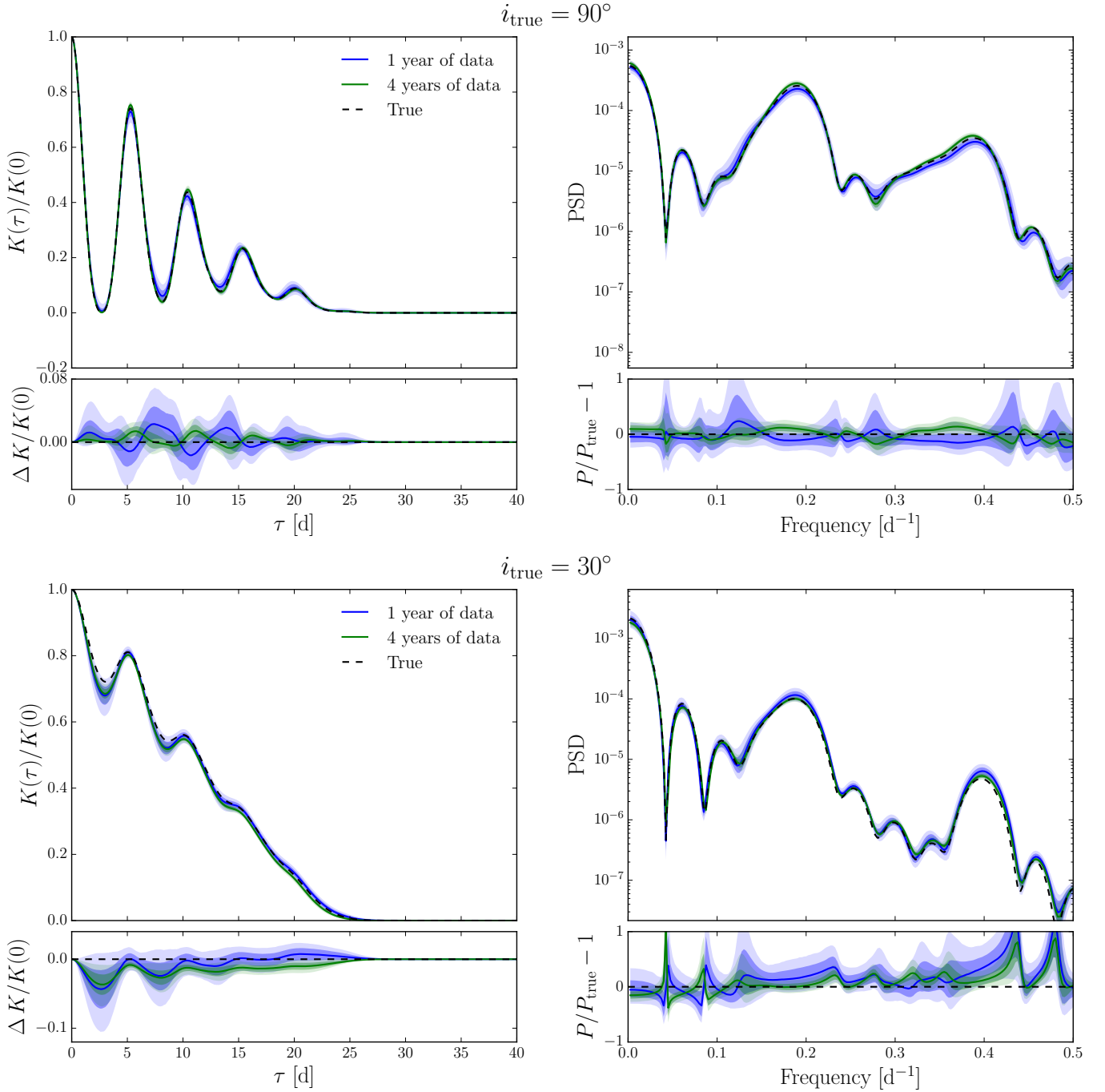
Figure 27. Kernel and PSD evaluated at 2000 random draws from the nested sampling posteriors in Figure 26, for I = 90^\circ (top) and I = 30^\circ (bottom). The left panels show the normalized kernel K(\tau)/K(0) , with each draw normalized by its own K(0) . The right panels show the PSD up to the Nyquist frequency of the \Delta t = 1 d sampling. Solid lines show the posterior median, and the dark and light shaded regions show the pointwise 68% and 95% intervals for 1 year (blue) and 4 years (green) of data. The dashed black lines show the kernel and PSD at the true parameters. The lower panels show the residuals from the truth: \Delta K/K(0) for the kernel and P/P_{\text{true}} - 1 for the PSD. The fractional PSD residual spikes near the nulls of the PSD, where P_{\text{true}} \rightarrow 0 .
