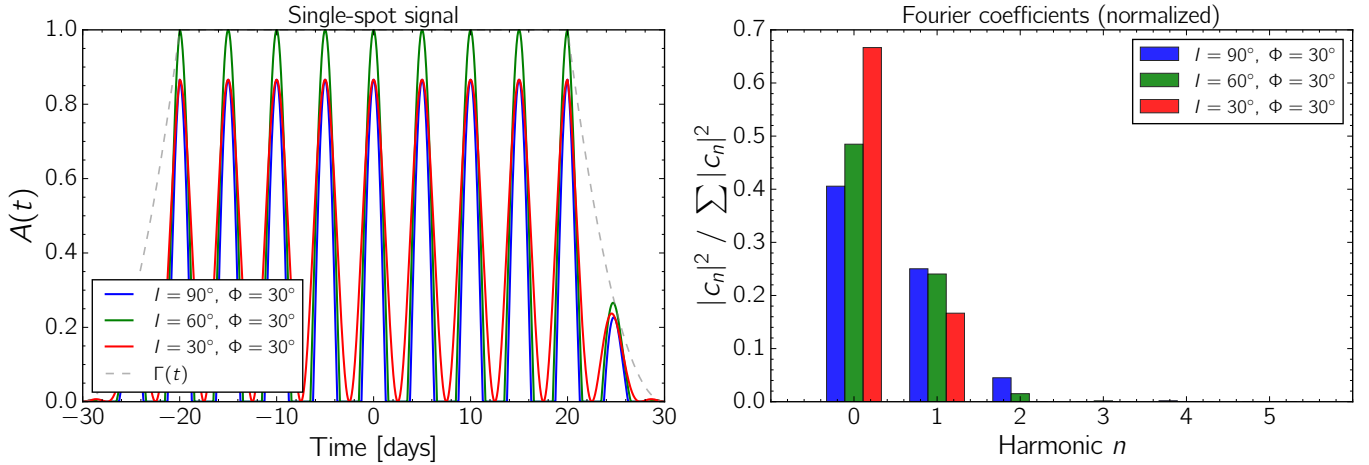
Figure 11. Fourier decomposition of the single-spot signal A(t) = \Gamma(t) \cdot \mathcal{V}(t) for a spot at latitude \Phi = 30^\circ . Left: Time-domain signal for three stellar inclinations, with the normalized squared envelope \Gamma(t) = \alpha^2(t)/\alpha_{\max}^2 shown as a dashed gray line. Right: Normalized squared Fourier coefficients |c_n|^2 / \sum |c_n|^2 of the visibility function for each inclination.
