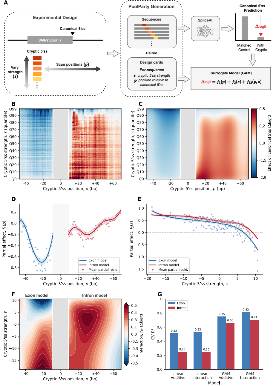
Fig. 4 Surrogate modeling of SpliceAI predictions. (A) Experimental design. Cryptic 5'ss 9-mers of varying MaxEntScan strength ( s ) were inserted at varying positions ( p ) flanking the canonical 5'ss of SMN2 exon 7. Each variant was paired with a control in which the splice-site GT dinucleotide is disrupted (GT→GA). PoolParty records the values of s and p in the design cards. The effect of each insertion on SpliceAI predictions at the canonical 5'ss is quantified as \Delta\text{logit} and modeled as a function of s and p using a generalized additive model (GAM). (B) Mean \Delta\text{logit} across the strength \times position grid (100 \times 100; each cell averages over 20 distinct 9-mers). The gray band marks the canonical 5'ss region. (C) GAM predictions (including the interaction term), using the same color scale as in B. (D) Partial dependence of the position term f_1(p) , shown separately for exon (blue) and intron (red) models. Shaded regions indicate 95% confidence intervals; points denote mean partial residuals. (E) Partial dependence of the strength term f_2(s) , with conventions as in D. (F) Interaction surface f_{12}(p, s) for exon and intron models. (G) Checkerboard cross-validation R^2 for linear and GAM models, with and without interaction terms.
