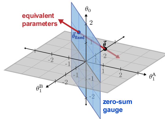
Fig. 1 Minimal example of gauge fixing. Shown is the three-dimensional space of parameter vectors [\theta_0, \theta_1^A, \theta_1^B] corresponding to an all-order model for sequences of length L = 1 built from the two-character alphabet \{A, B\} . Black dot: the parameter vector \vec{\theta} = [0, 0, 2] . Red line: parameter vectors equivalent to \vec{\theta} . Blue plane: parameter vectors in the zero-sum gauge, i.e., those satisfying \theta_1^A + \theta_1^B = 0 . Blue dot: gauge-fixed parameters \vec{\theta}_{\text{fixed}} = [1, -1, 1]
