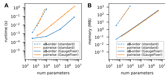
Fig. 2 Benchmarking results. Shown are the runtime (A) and peak memory (B) requirements for GaugeFixer and for standard matrix multiplication, plotted as a function of the number of model parameters. Tests were carried out for all-order models ( L = 2 to 5 ) and pairwise models ( L = 3 to 150 ) on protein sequences ( \alpha = 20 ). Each data point represents the mean and standard deviation over 10 gauge-fixing computations performed on a standard laptop computer. No execution-time limit was imposed, but benchmarking computations for standard matrix multiplication were restricted to models whose projection matrix required less than 2 GB of memory.
