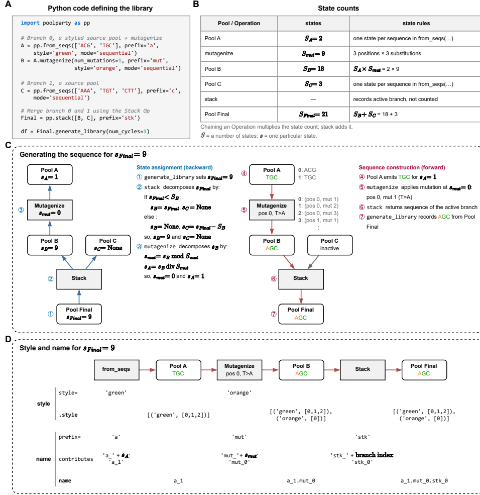
Fig. 1 A worked example of sequence generation. (A) Python code defining the library. (B) Number of states of each Pool and Operation. (C) Generating the sequence for s_{Final} = 9 . Left: state assignment (blue). Right: sequence construction (magenta). Lists beside Pool A and mutagenize show which sequence or mutation each state selects. Inactive branches are shown in grey. (D) Style and name for the same sequence. Sequences are carried through the DAG as Seq objects, which hold the sequence string together with its .style . The style and prefix arguments are supplied to Operations; the resulting .style and name are held by Pools. Sequence characters are colored by their .style entries; where entries overlap, the last one applies.
