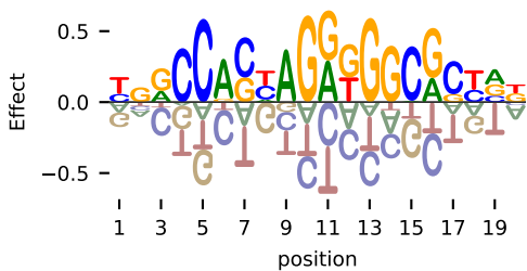
(c) MAX ( L = 11, C = 4 )
