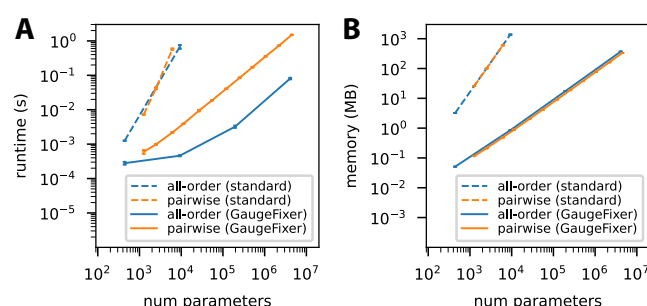
Fig. 2. Benchmarking results. Shown are the runtime (A) and peak memory (B) requirements for GaugeFixer and for standard matrix multiplication, plotted as a function of the number of model parameters. Tests were carried out for all-order models ( L = 2 to 5 ) and pairwise models ( L = 3 to 150 ) on protein sequences ( \alpha = 20 ). Each data point represents the mean and standard deviation over 10 gauge-fixing computations performed on a standard laptop computer. No execution-time limit was imposed, but benchmarking computations for standard matrix multiplication were restricted to models whose projection matrix required less than 2 GB of memory.
