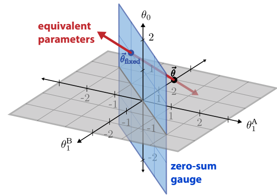
Fig. 1. Minimal example of gauge fixing. Shown is the three-dimensional space of parameter vectors [\theta_0, \theta_1^A, \theta_1^B] , corresponding to an all-order model for sequences of length L = 1 built from the two-character alphabet \{A, B\} . Black dot: the parameter vector \vec{\theta} = [0, 0, 2] . Red line: parameter vectors equivalent to \vec{\theta} . Blue plane: parameter vectors in the zero-sum gauge, i.e., those satisfying \theta_1^A + \theta_1^B = 0 . Blue dot: gauge-fixed parameters \vec{\theta}_{\text{fixed}} = [1, -1, 1] .
