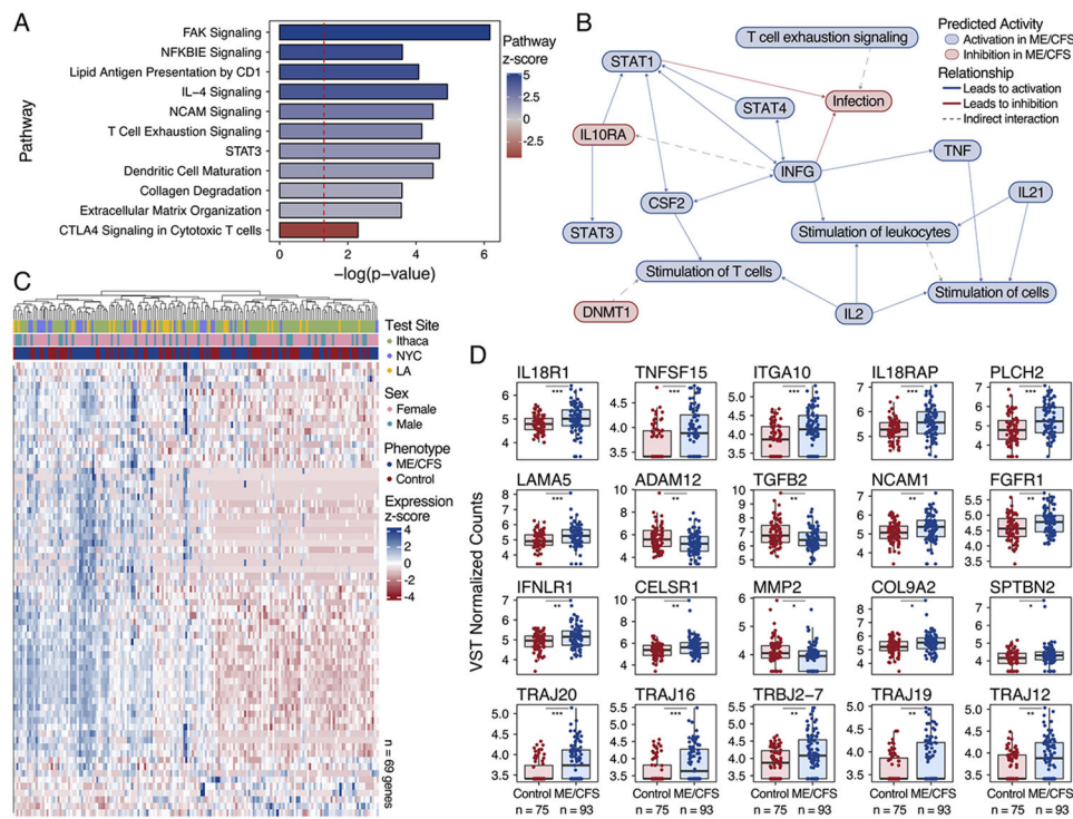
Fig. 4. Biological pathway analysis of ME/CFS. (A) Top 10 most significantly activated (blue) pathways and most significantly inhibited (red) pathways in cases as determined by -\log(P\text{-value}) and a nonzero z-score. (B) Network analysis of the predicted pathways of ME/CFS (Qiagen, IPA). (C) Heatmap of activated (blue) and inhibited (red) pathway marker genes for the selected pathways (n = 69 genes). (D) VST counts of the top 20 most significantly differentially pathway marker genes between controls and cases ( P\text{-adj} values as follows; * P < 0.05 , ** P < 0.01 , *** P < 0.005 ).
