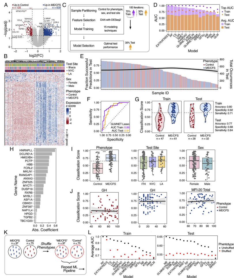
Fig. 2. Machine learning for ME/CFS classification. (A) Volcano plot of differential abundance analysis of exercise-independent cfRNA between cases and controls (DESeq2). 608 transcripts are elevated in cases (blue, BH adjusted P -values ( P -adj) < 0.05 , \log_2\text{FoldChange} > 0.5 ) and 135 transcripts are elevated in controls (red, P -adj < 0.05 , \log_2\text{FoldChange} < -0.5 ). (B) Variance stabilizing transformation (VST) values of significantly differentially abundant genes ( n = 281 genes, P -adj < 0.05 , \text{abs}(\log_2\text{FoldChange}) > 0.75 ) between phenotypes. Samples and genes are clustered based on correlation. (C) Workflow of machine learning pipeline. (D) Bar chart of average performance across 100 iterations for each machine learning model for train (purple) and test (orange) sets. Dots indicated the top-performing iteration for each model. (E) Fraction of successful classification for each subject in the test set (left y -axis). Number of times each sample is assigned to the test set (right y -axis) shown by a LOESS smoothed line (black) across samples color coded by phenotype. (F) AUC-ROC plot of model performance for one GLMNET Lasso train (purple) and test (orange) set distinguishing cases from controls. (G) Violin plots of classifier scores for training (specificity: 0.92, sensitivity: 0.71, accuracy: 0.80) and test sets (specificity: 0.68, sensitivity: 0.84, accuracy: 0.77). Youden threshold cutoff (0.65) shown with dashed line. (H) 21 gene features selected by the GLMNET Lasso ranked by absolute coefficient. (I) Comparison of model performance and phenotype ( ***P < 1e - 12 ), test site, and sex.
