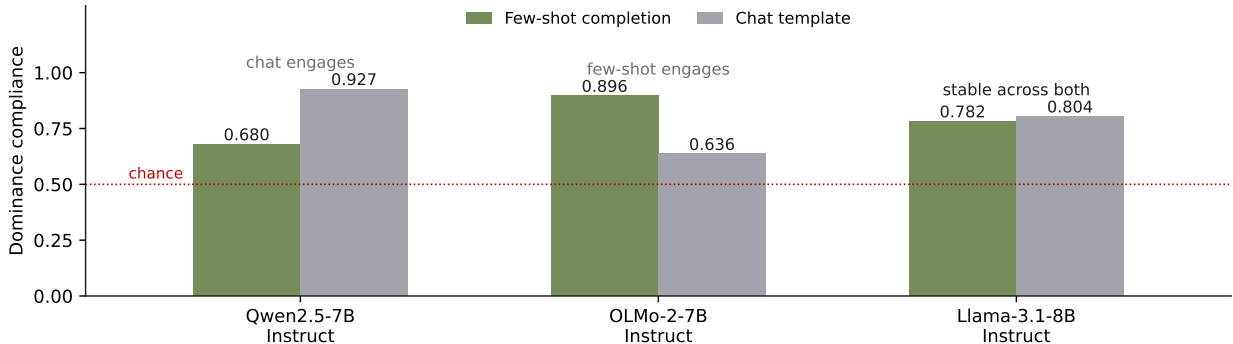
Figure 2: Dominance compliance by elicitation format for the three instruct models. Which format elicits an engaged subject reverses between Qwen and OLMo, and Llama is stable across both. The same weights score 0.680 or 0.927 depending only on how the prompt is packaged, so format is part of the measurement rather than a neutral container for it.
