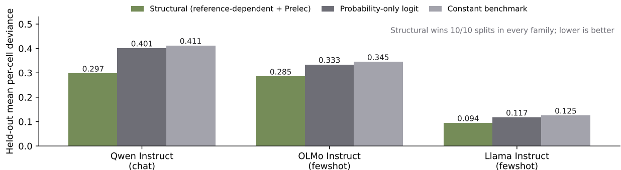
Figure 4: Held-out mean per-cell deviance on gambles the fit never saw, averaged over 10 random 30/10 splits. The structural model beats the probability-only reduced form in every family and on every individual split, and the constant benchmark trails both. Phase 1’s in-sample near-tie between the structural model and the probability-only logit does not survive out of sample.
