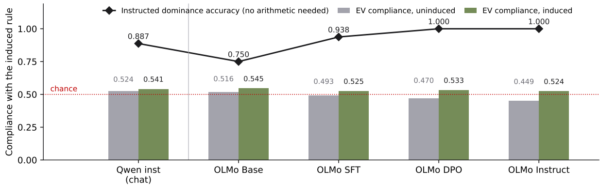
Figure 3: Compliance with an instructed decision rule, by what the rule demands. The bars are expected-value compliance on cells where following the rule requires multiplying p by h : uninduced against induced, both hugging chance at every training stage. The line is accuracy on the dominant controls under the same instruction, where the induced optimum requires no arithmetic, reaching 1.000 by DPO. Post-training buys instruction-following on the cells that need no computation and does not buy the computation.
