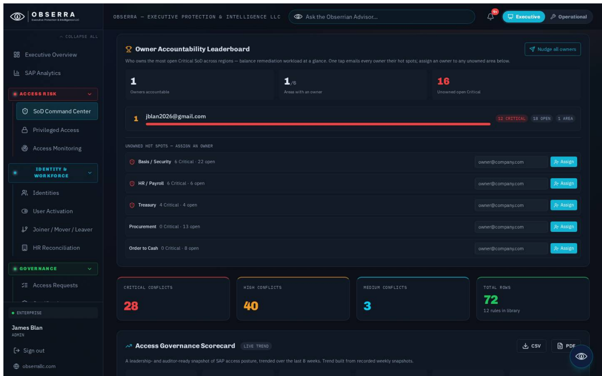
Figure: 8. Risk Watchlist, Owner Leaderboard & Board Pack
