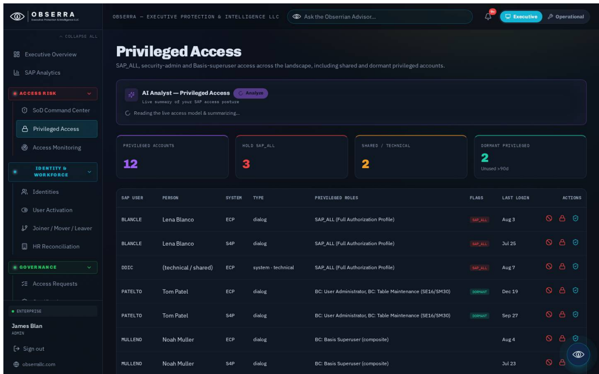
Figure 9. Privileged Access (PAM)
