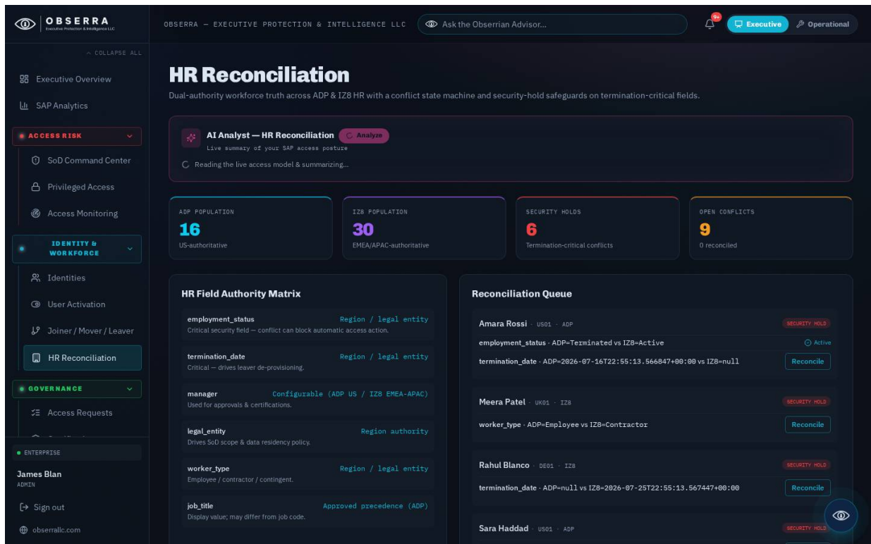
Figure: 13. HR Reconciliation
