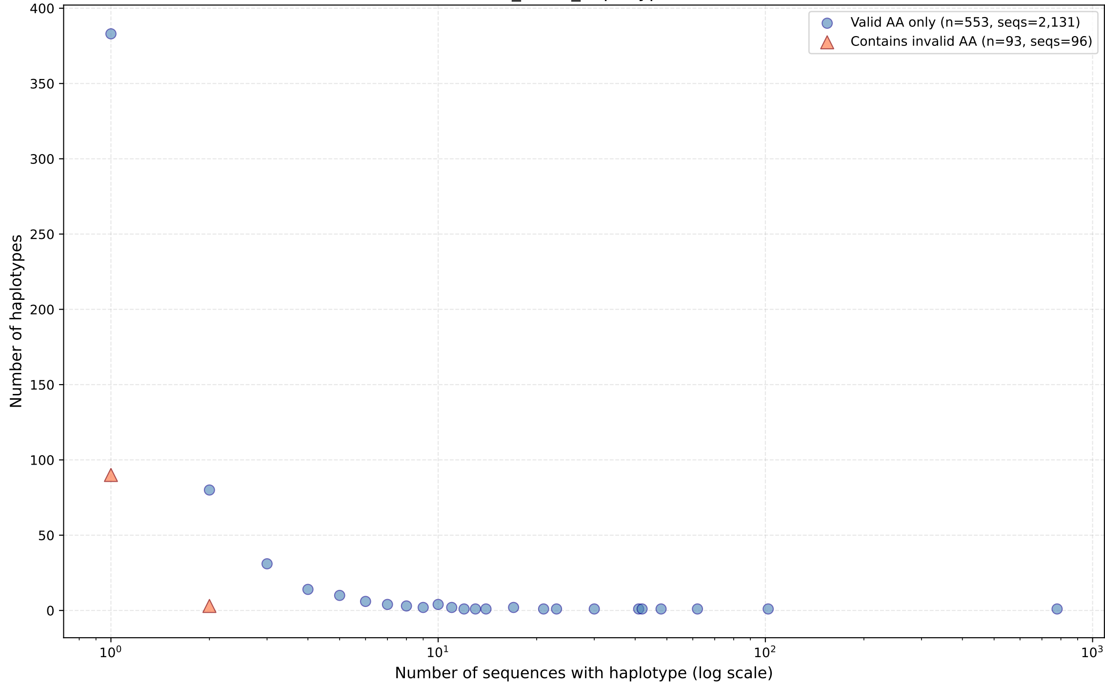
Distribution of Haplotype Counts recent_H3N2_haplotypes.tsv
