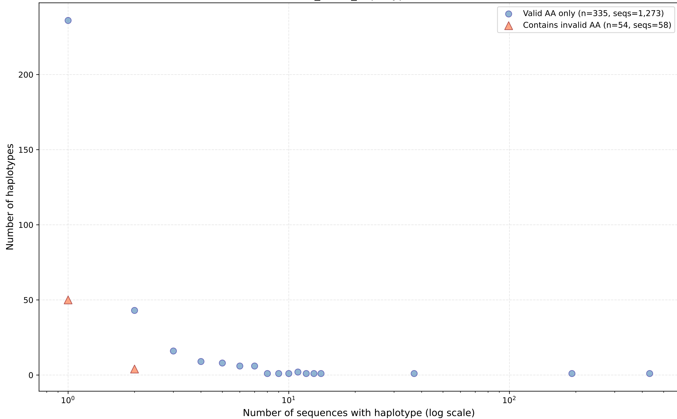
Distribution of Haplotype Counts recent_H1N1_haplotypes.tsv
