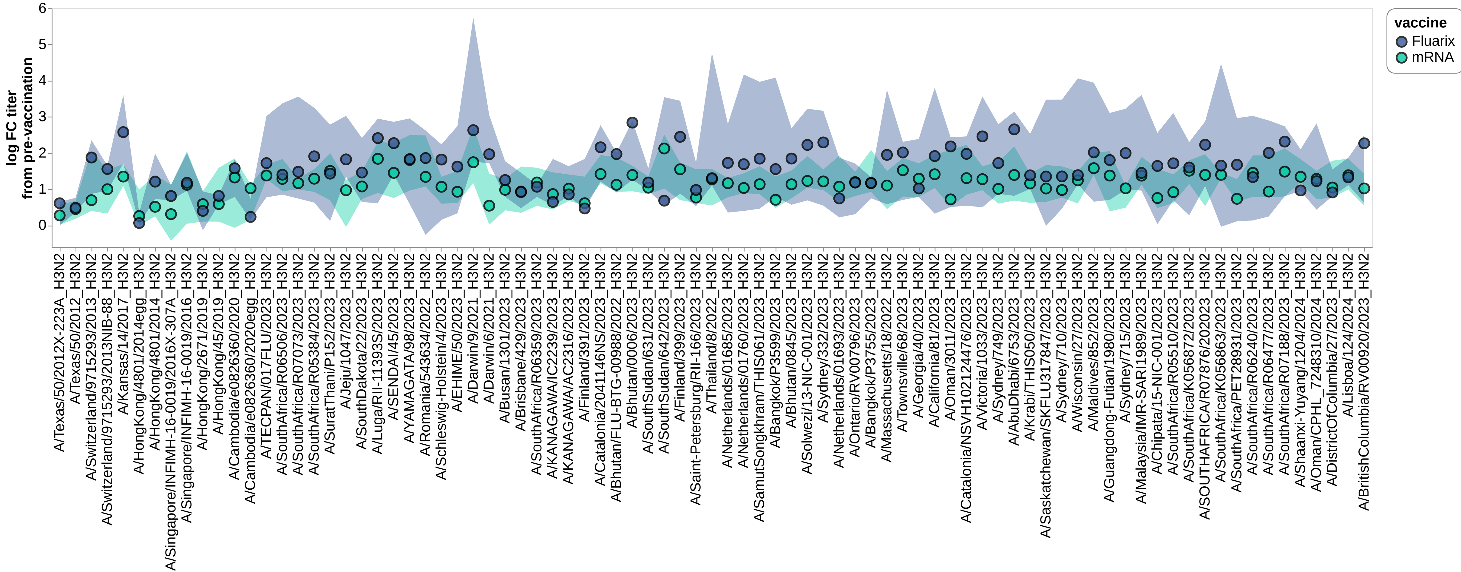
Log FC day 29 titers to H3N2 2023-2024 circulating strains and recent vaccine strains
