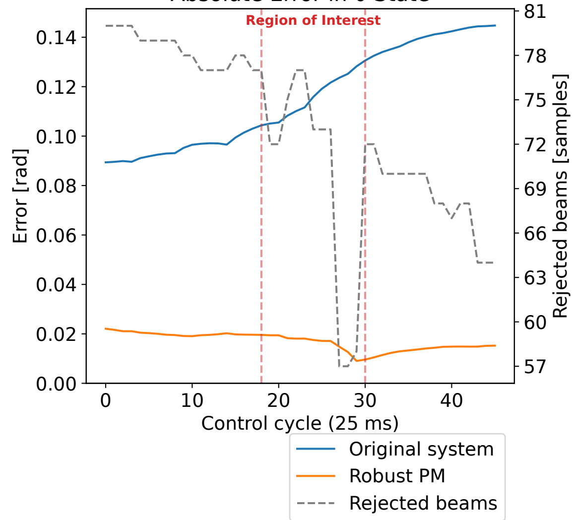
Absolute Error in \theta State
