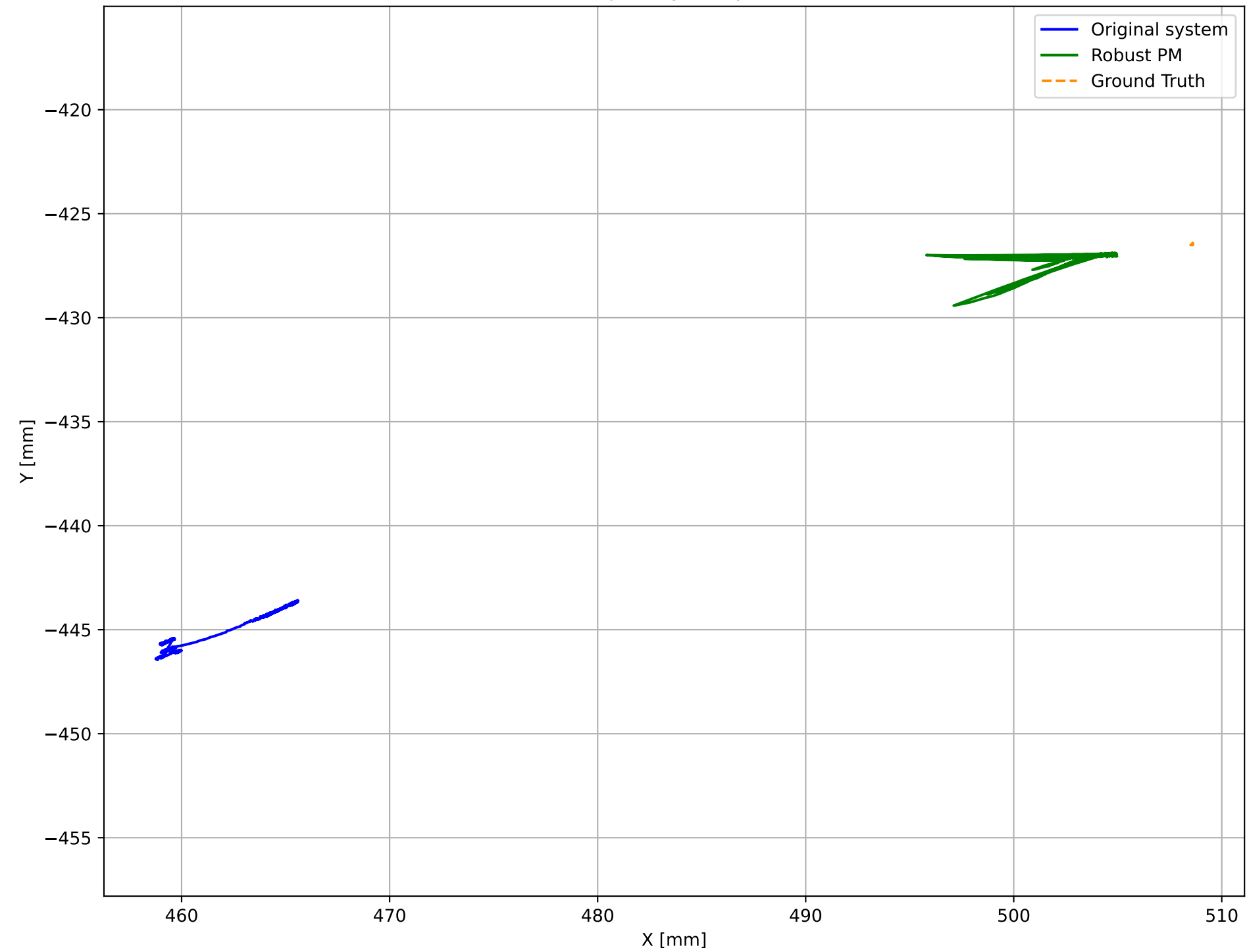
EKF trajectory comparison
