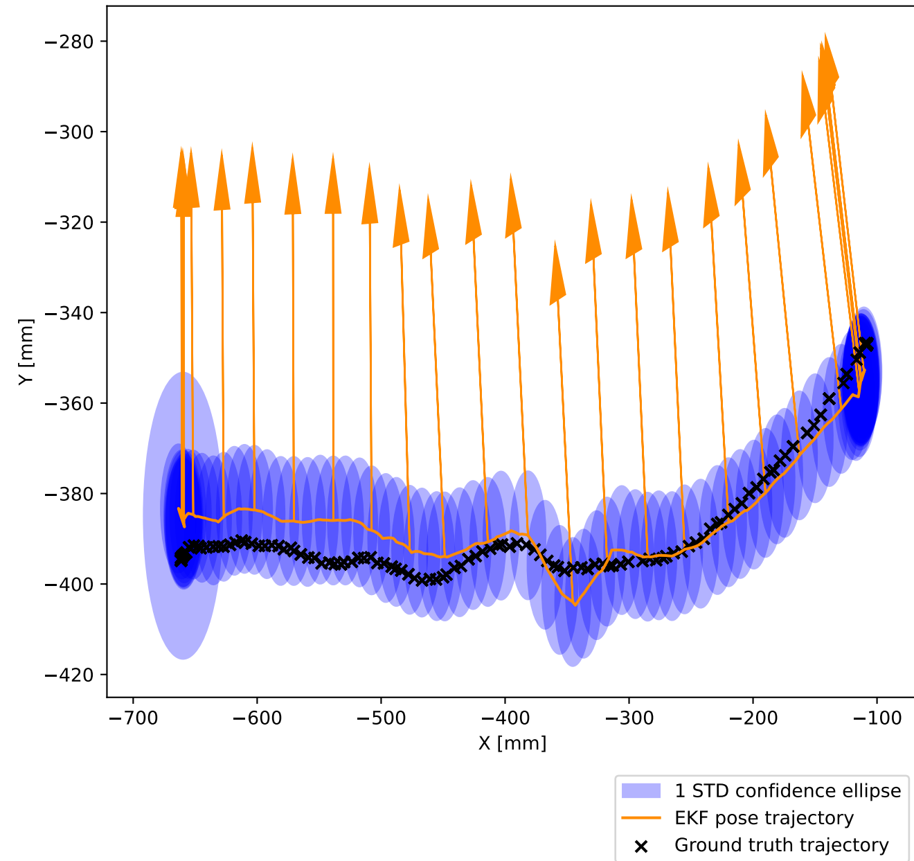
Robust PM
