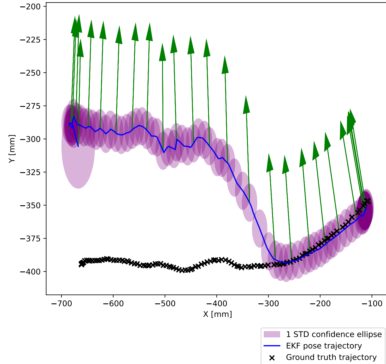
Original system
