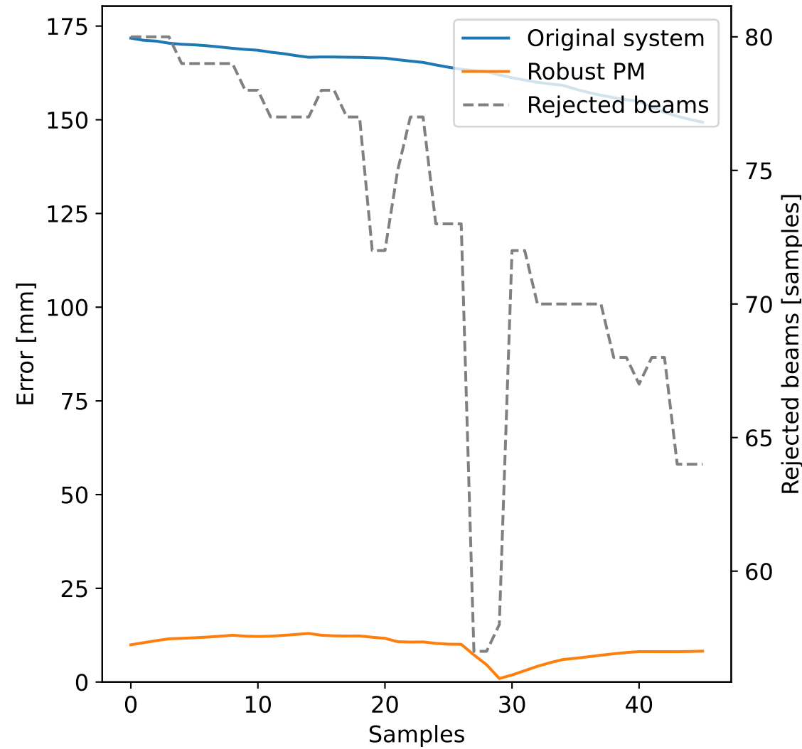
Absolute Error in Y State
