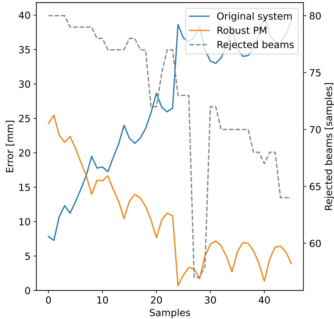
Absolute Error in X State
