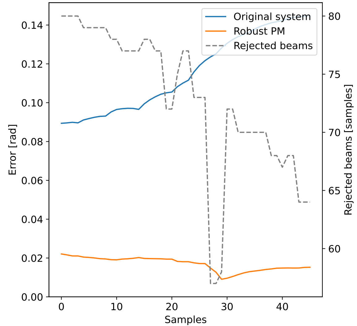
Absolute Error in \theta State
