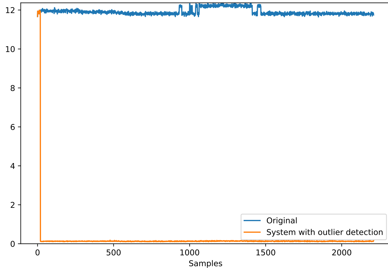
Error in PM [mm]
