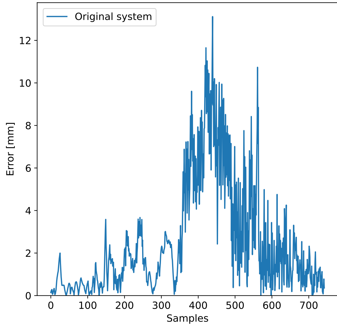
Absolute Error in X State
