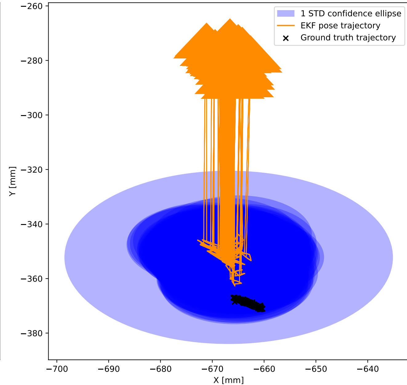
Robust PM
