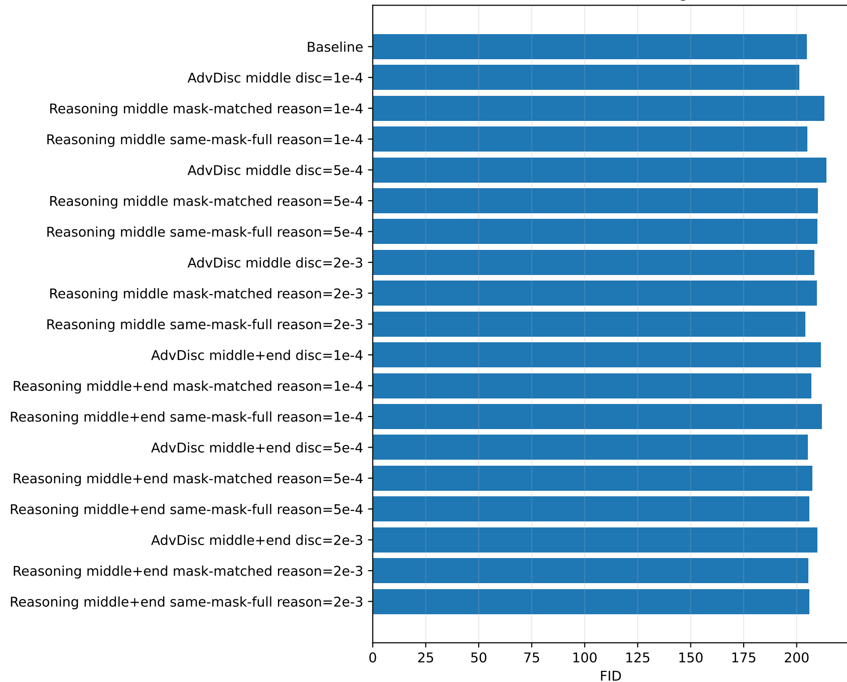
Advanced Discriminator and Reasoning Guidance: Final FID
