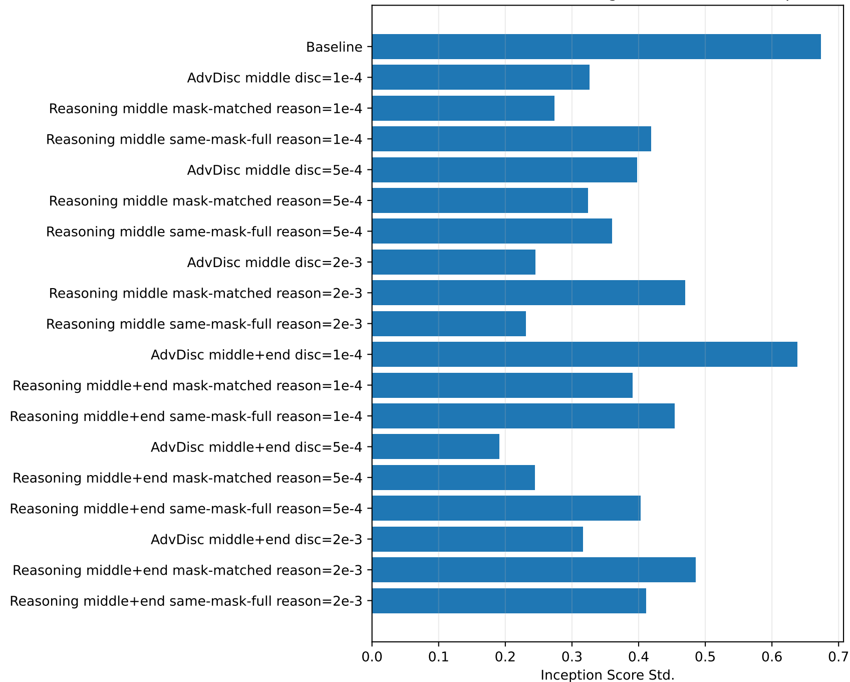
Advanced Discriminator and Reasoning Guidance: Final Inception Score Std.
