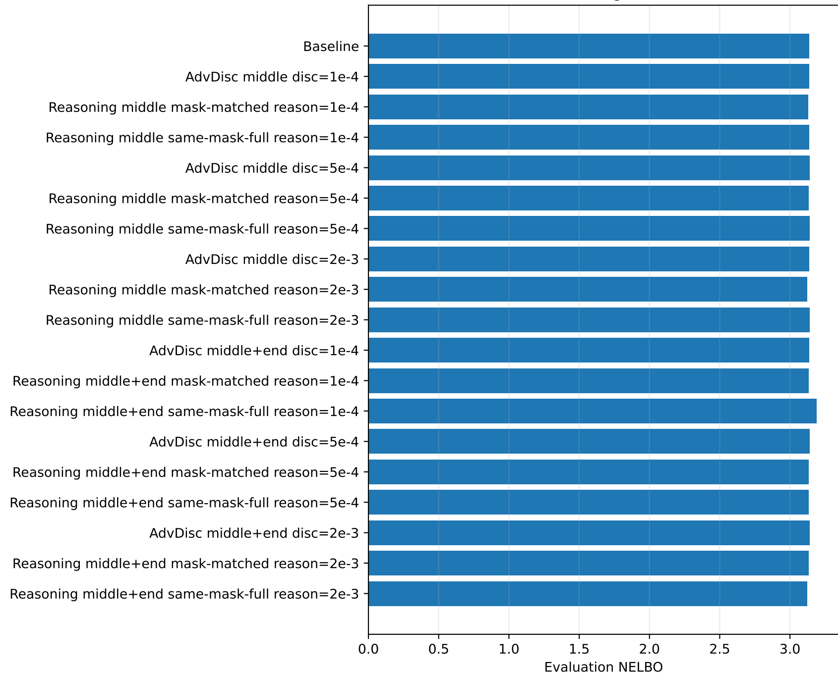
Advanced Discriminator and Reasoning Guidance: Final Evaluation NELBO
