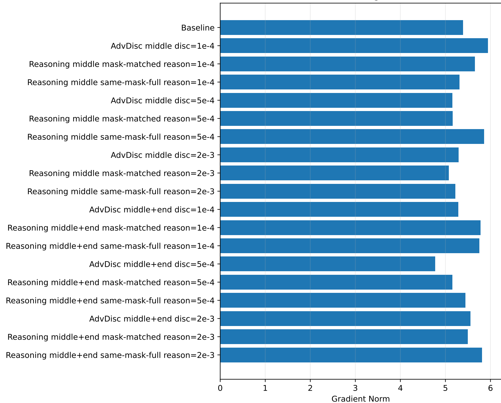
Advanced Discriminator and Reasoning Guidance: Final Gradient Norm
