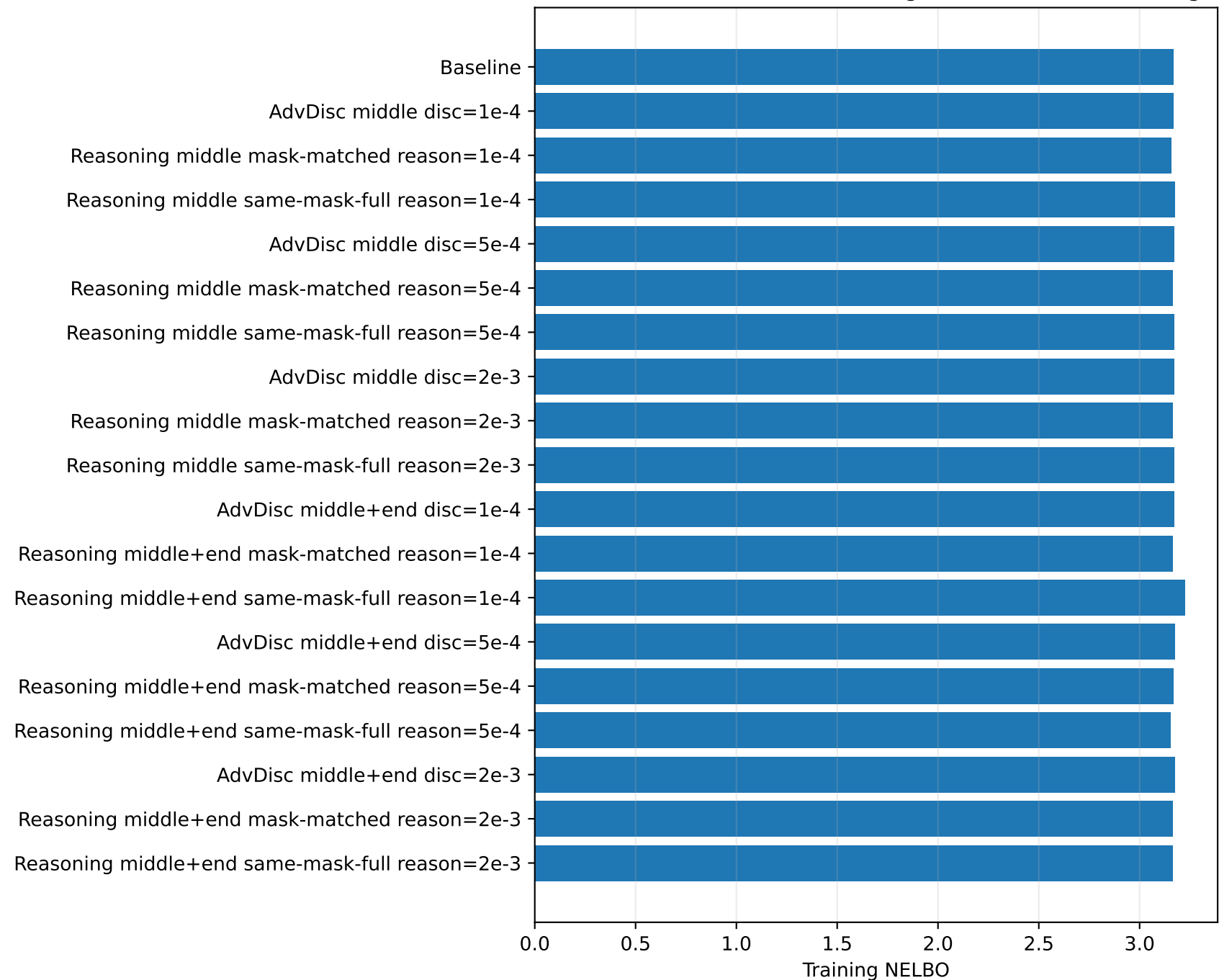
Advanced Discriminator and Reasoning Guidance: Final Training NELBO
