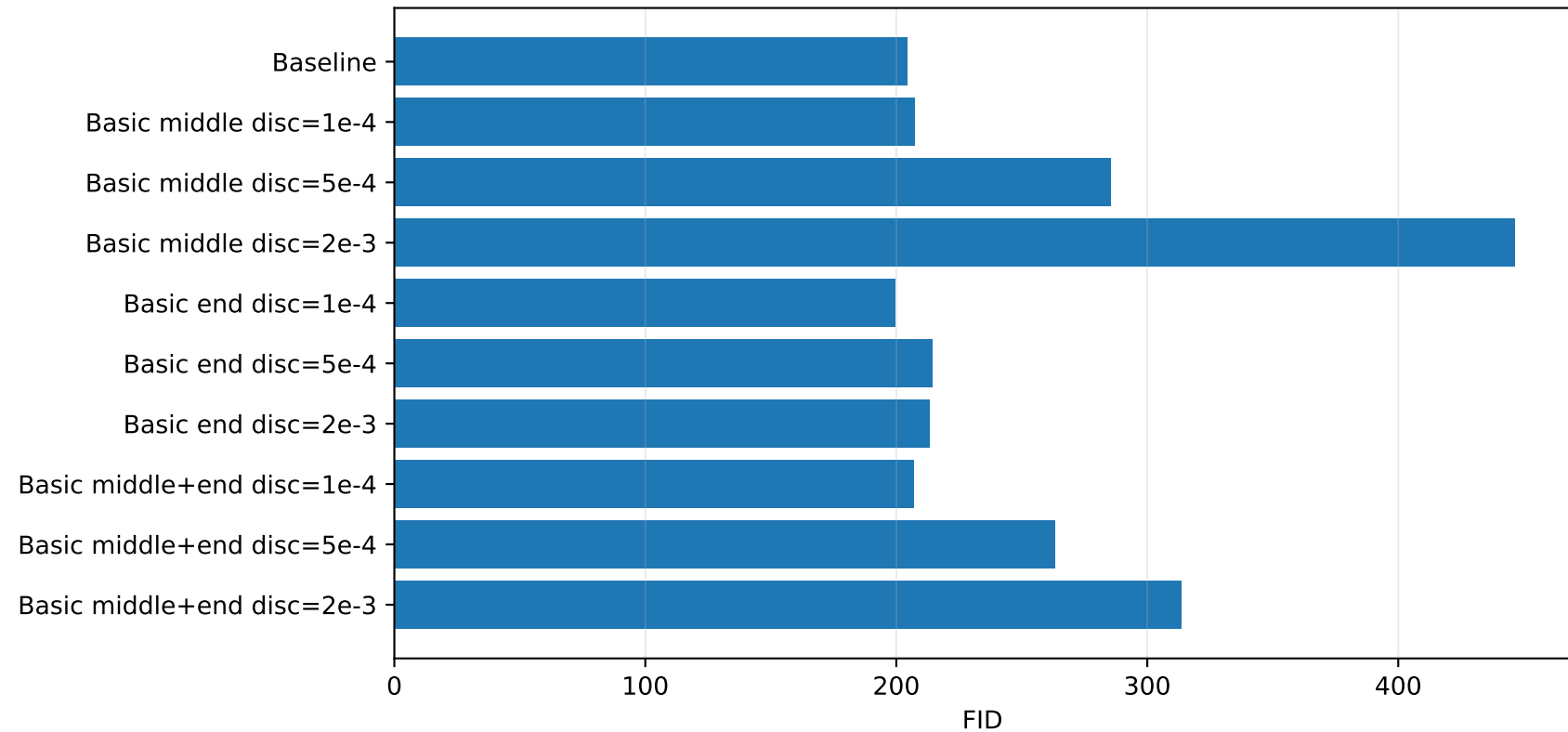
Basic Discriminator Guidance: Final FID
