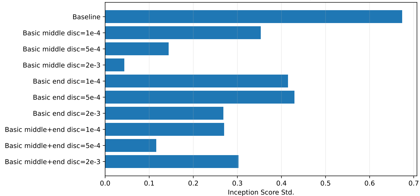
Basic Discriminator Guidance: Final Inception Score Std.
