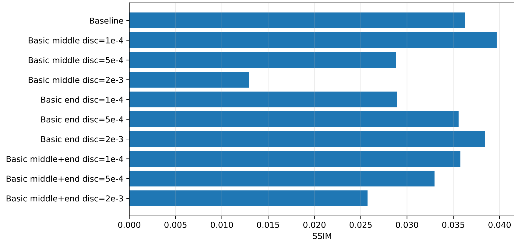
Basic Discriminator Guidance: Final SSIM
