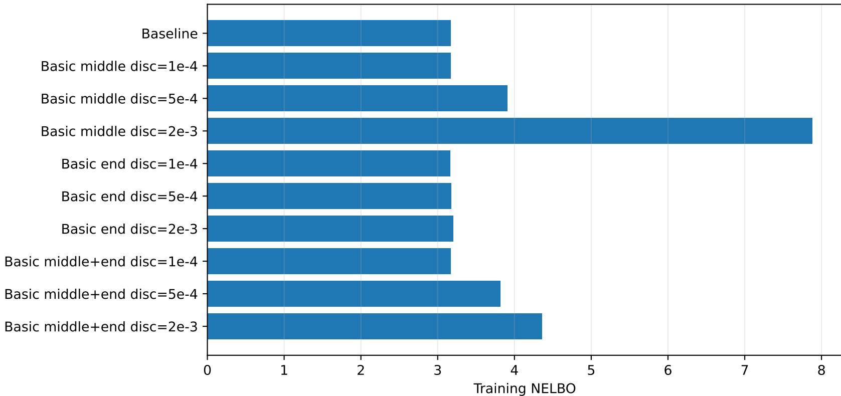
Basic Discriminator Guidance: Final Training NELBO
