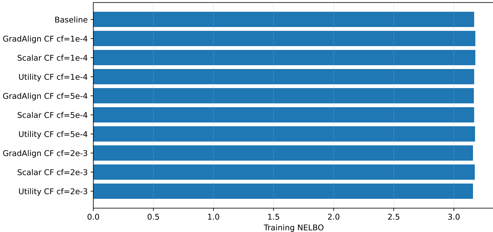
Counterfactual Feature-Credit Guidance: Final Training NELBO
