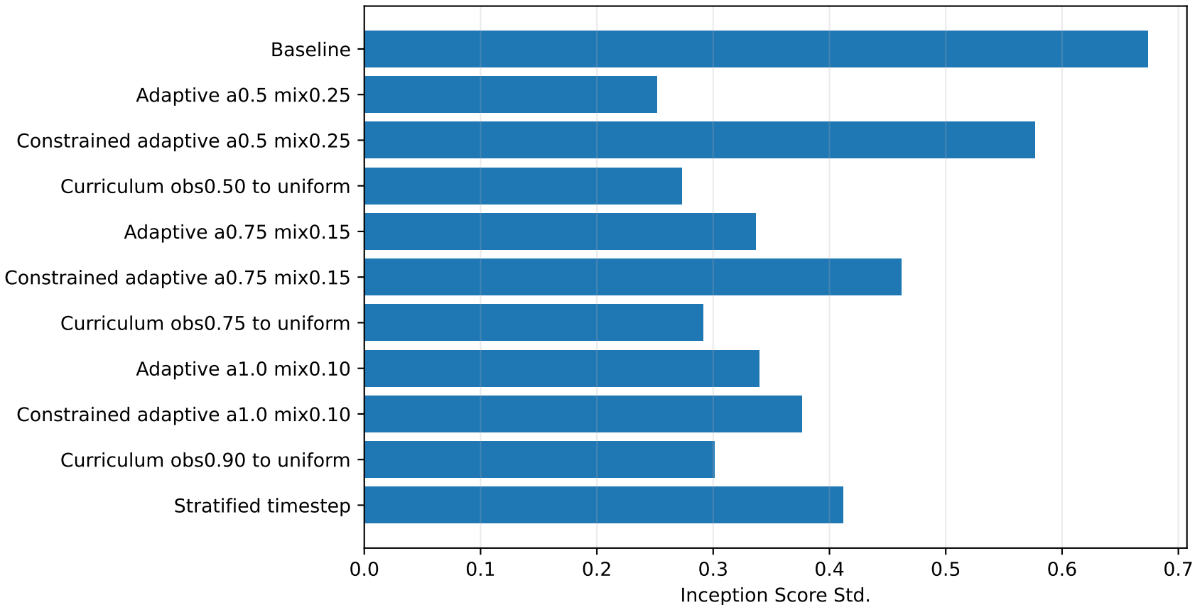
Scheduling-Based ARDM: Final Inception Score Std.
