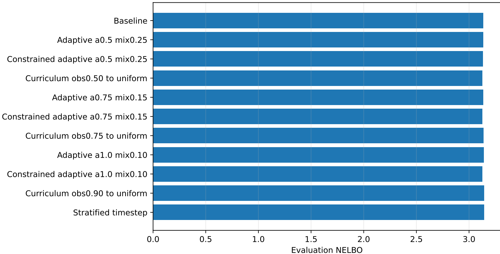
Scheduling-Based ARDM: Final Evaluation NELBO
