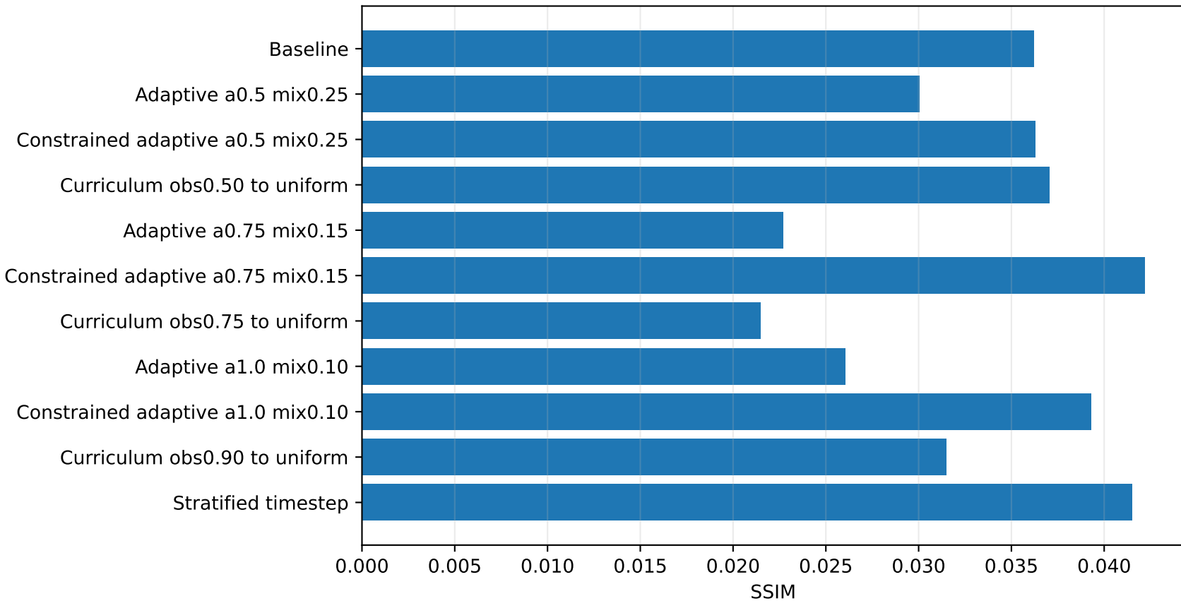
Scheduling-Based ARDM: Final SSIM
