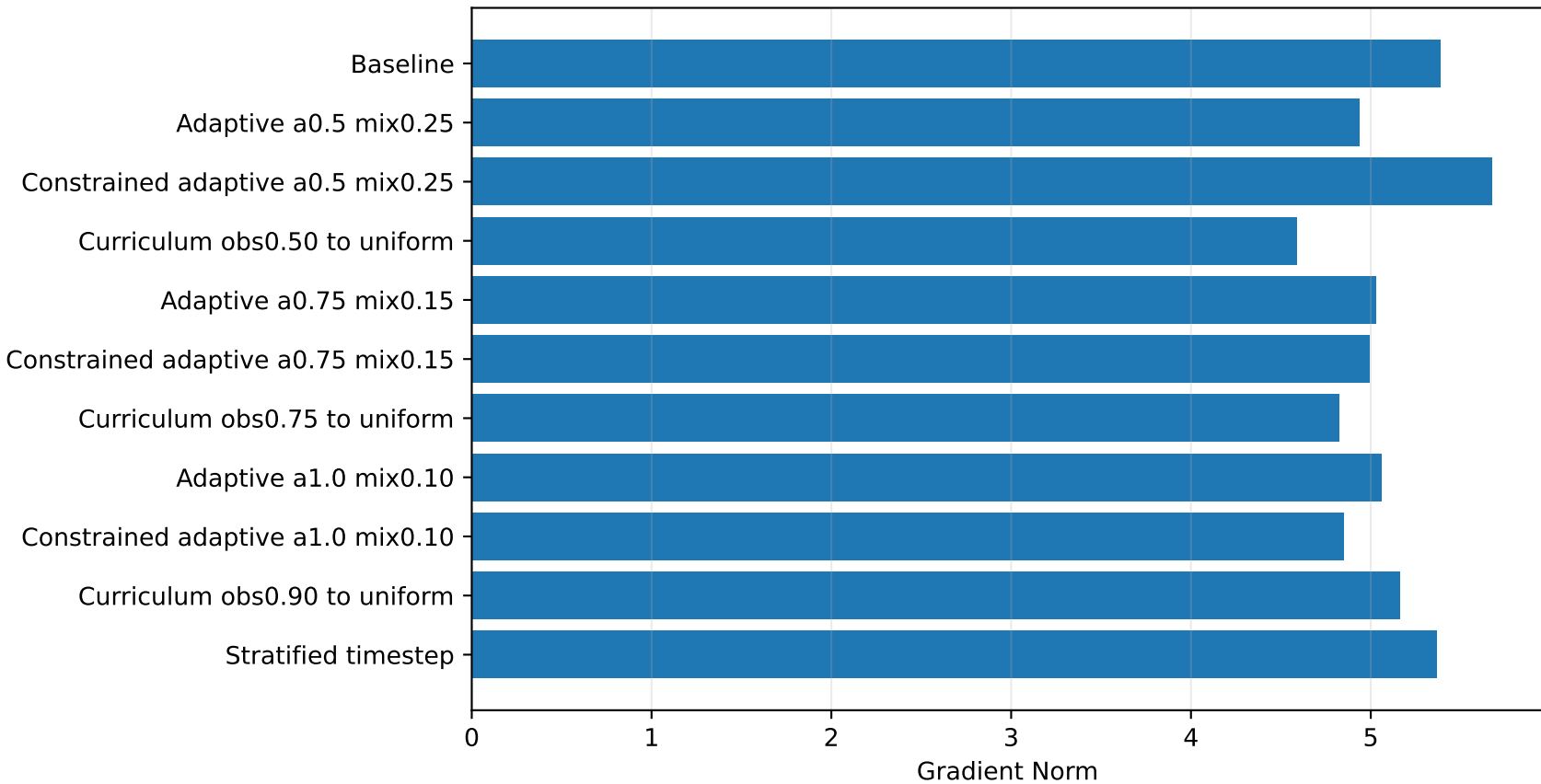
Scheduling-Based ARDM: Final Gradient Norm
