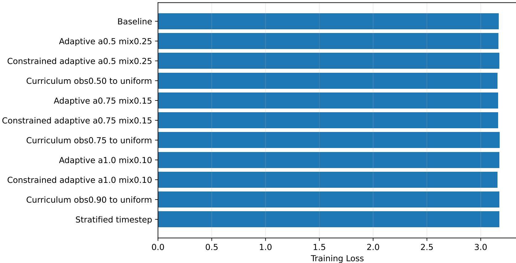
Scheduling-Based ARDM: Final Training Loss
