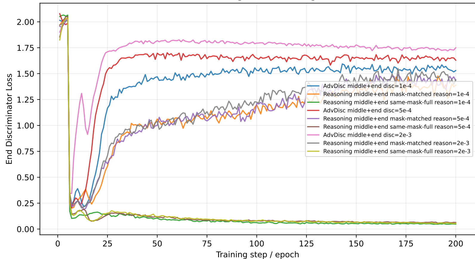
Advanced Discriminator and Reasoning Guidance Diagnostic: End Discriminator Loss
