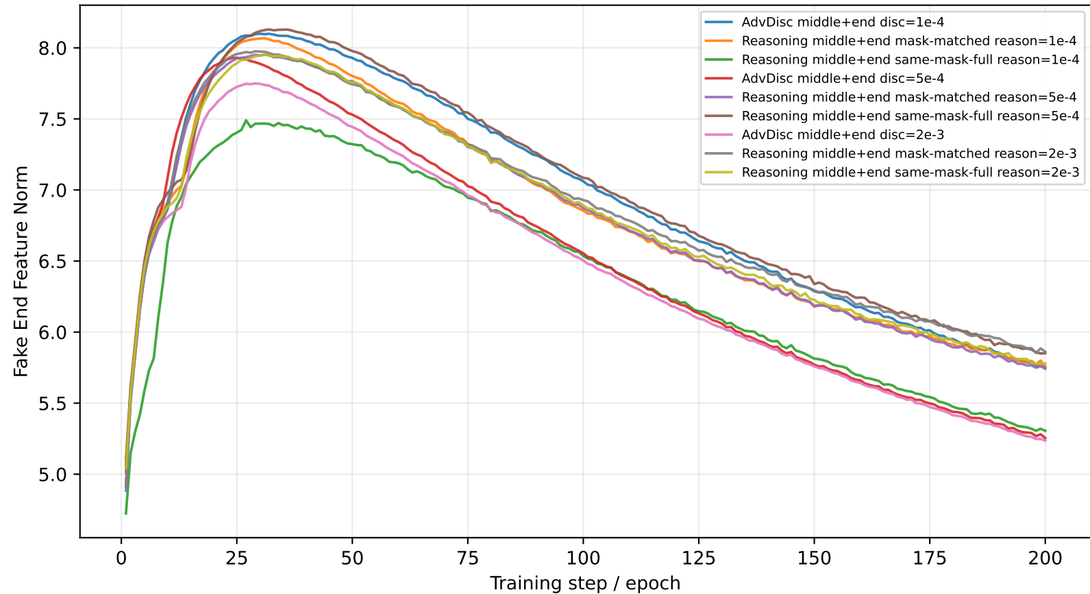
Advanced Discriminator and Reasoning Guidance Diagnostic: Fake End Feature Norm
