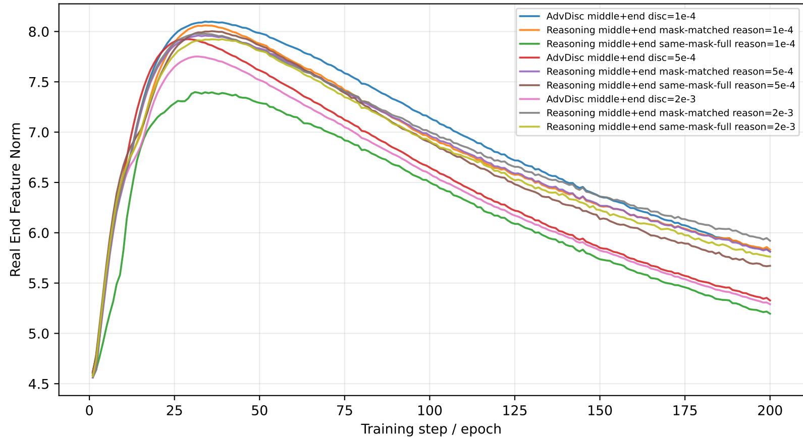
Advanced Discriminator and Reasoning Guidance Diagnostic: Real End Feature Norm
