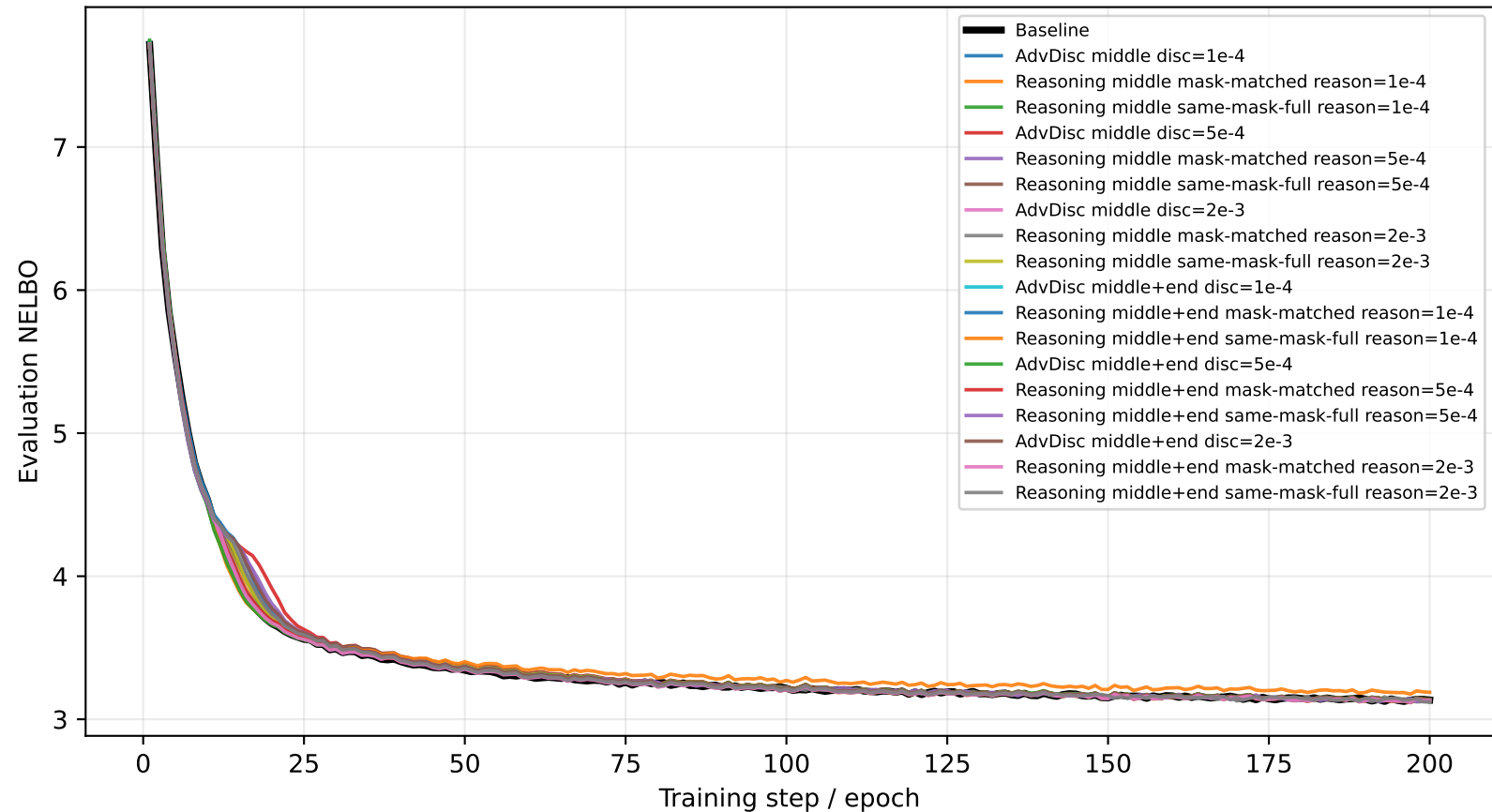
Advanced Discriminator and Reasoning Guidance: Evaluation NELBO
