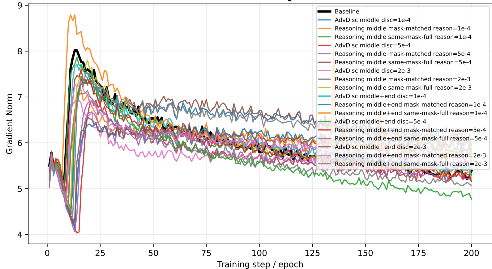
Advanced Discriminator and Reasoning Guidance: Gradient Norm
