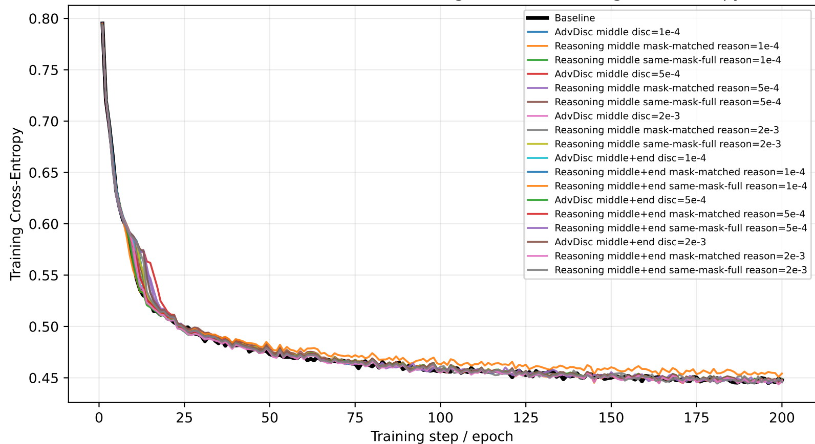
Advanced Discriminator and Reasoning Guidance: Training Cross-Entropy
