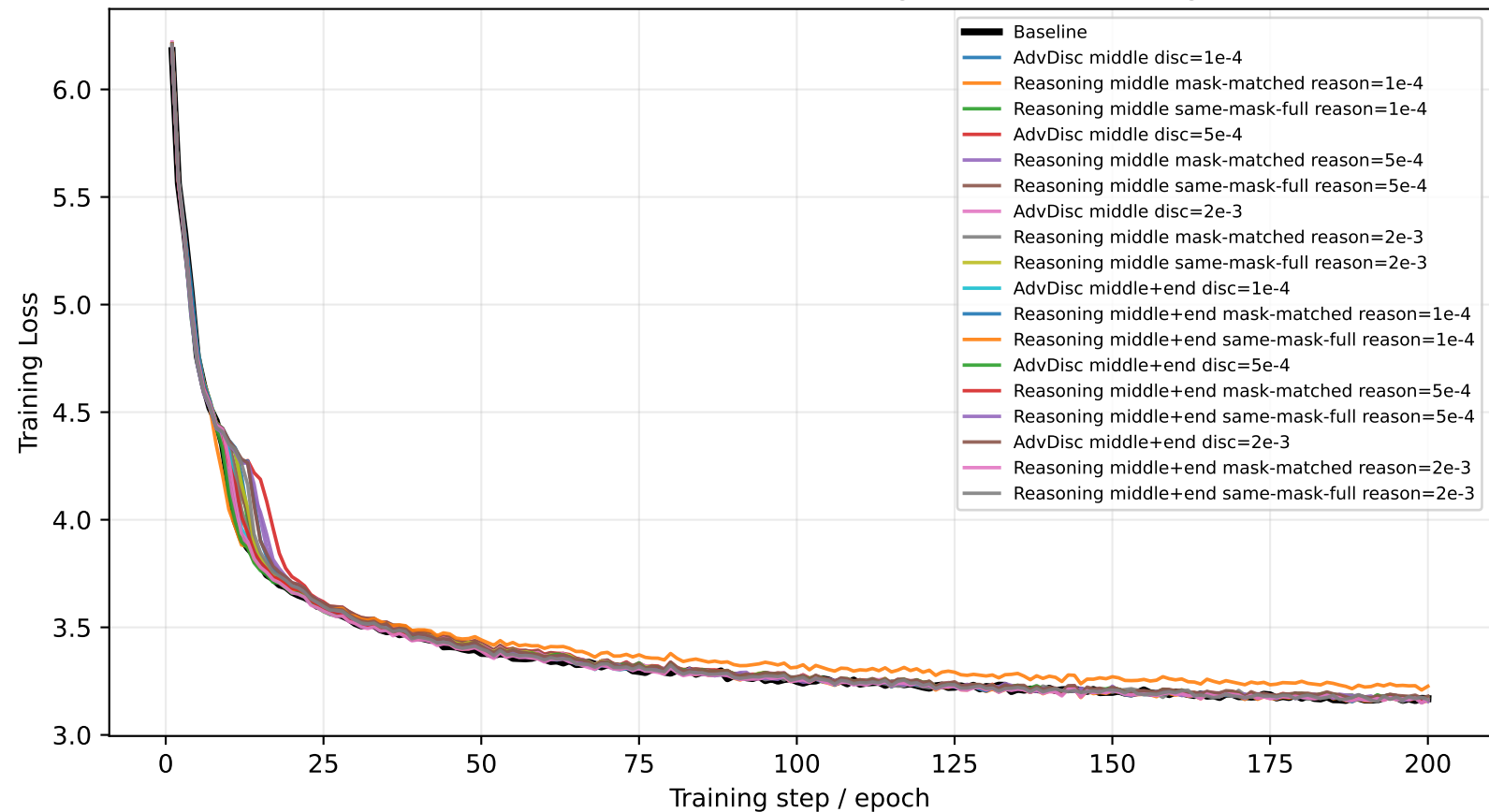
Advanced Discriminator and Reasoning Guidance: Training Loss
