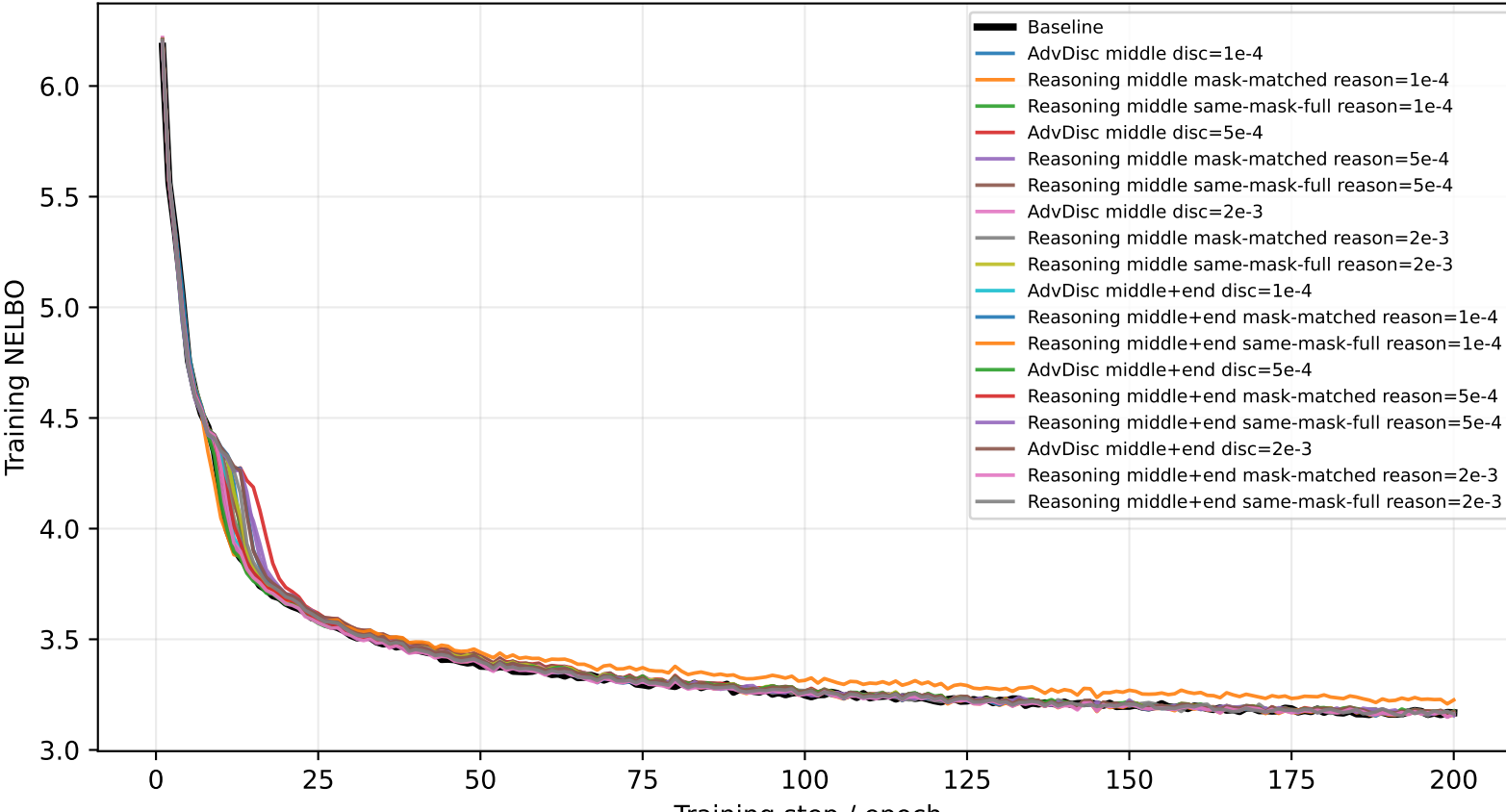
Advanced Discriminator and Reasoning Guidance: Training NELBO
