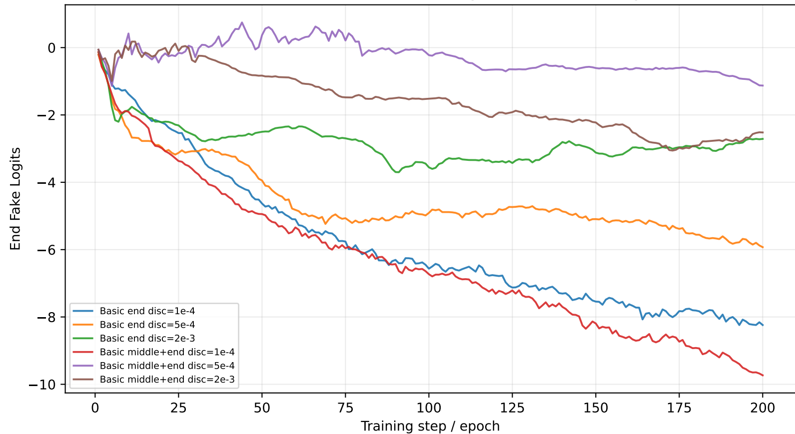
Basic Discriminator Guidance Diagnostic: End Fake Logits
