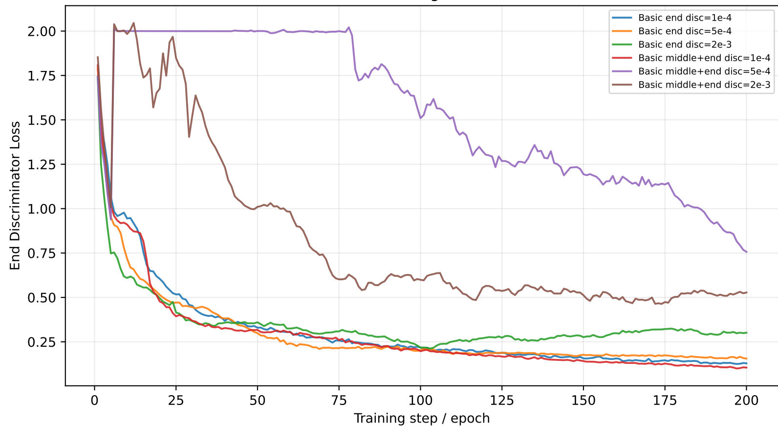
Basic Discriminator Guidance Diagnostic: End Discriminator Loss
