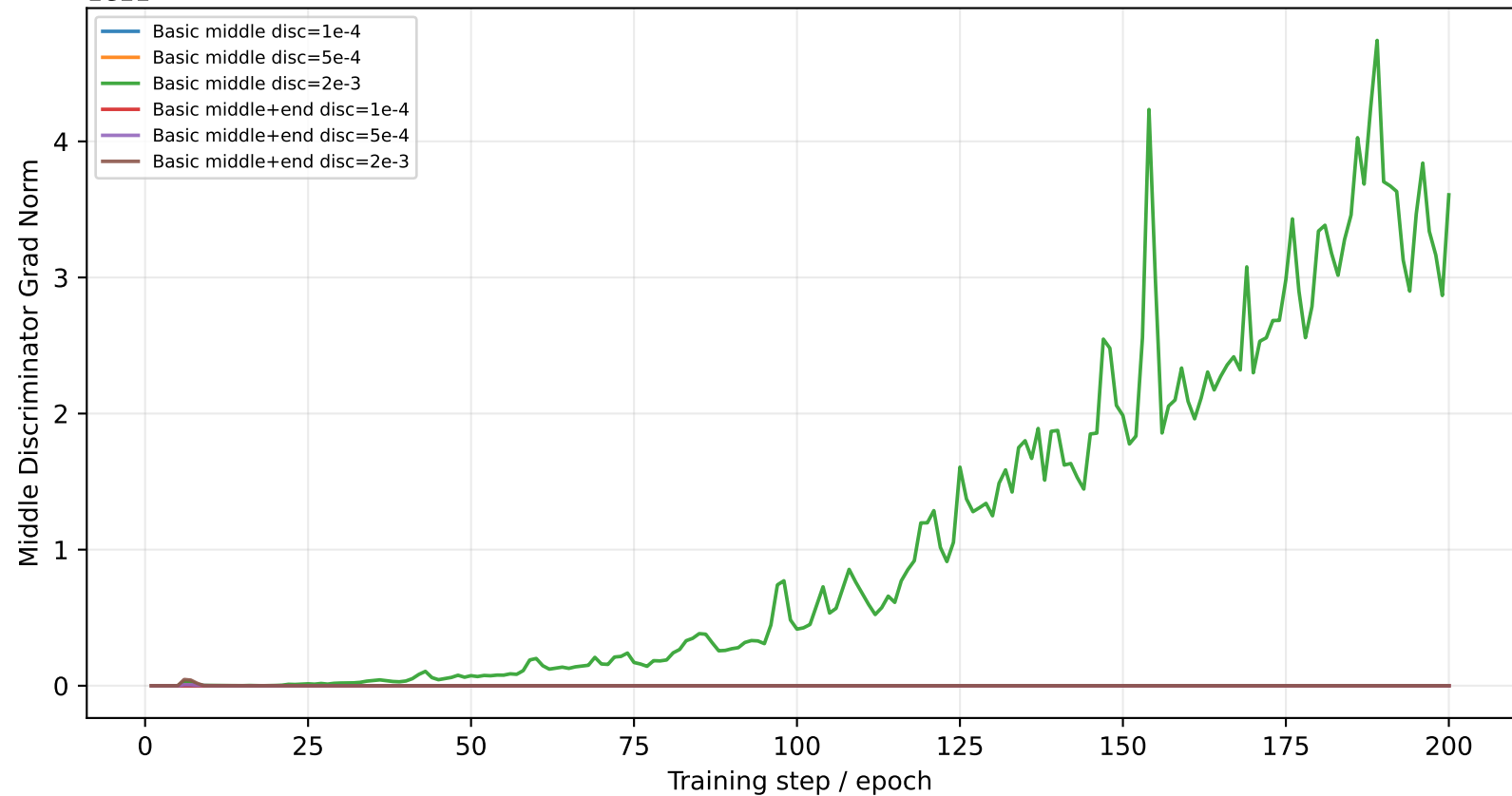
1e11 Basic Discriminator Guidance Diagnostic: Middle Discriminator Grad Norm
