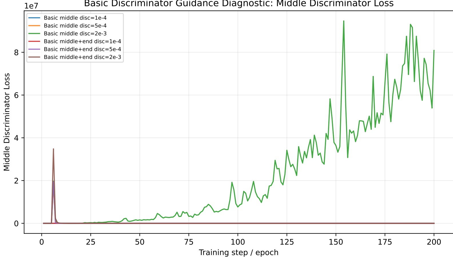
Basic Discriminator Guidance Diagnostic: Middle Discriminator Loss
