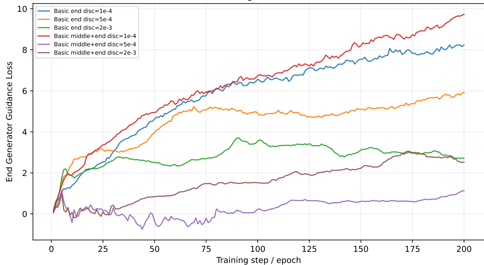
Basic Discriminator Guidance Diagnostic: End Generator Guidance Loss
